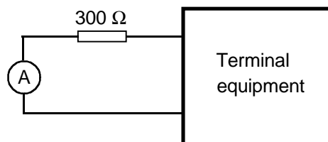
Figure A.10: Power feeding test for 2 wire TE
