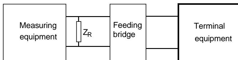
Figure A.8: Sending level between 4,3 kHz and 200 kHz configuration
