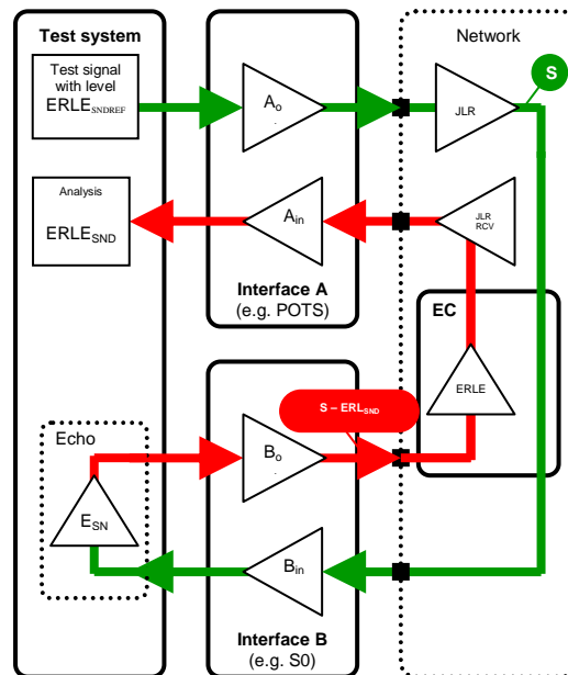
Figure B.2: Measurement setup for echo simulation
