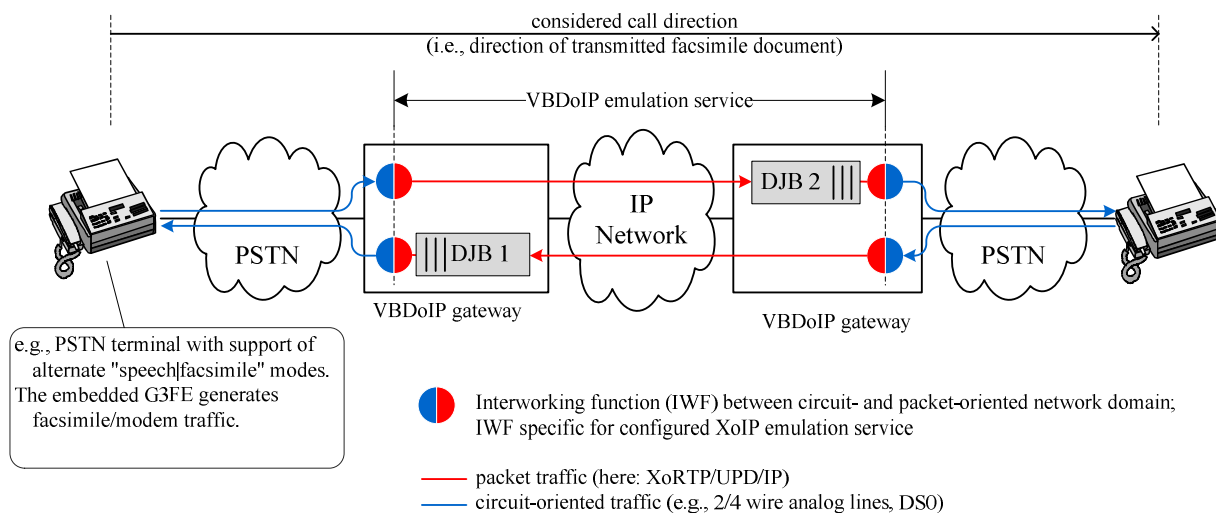
Figure 12: Example of a VBDiP emulation service
