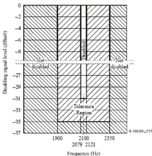
Figure 19: Required disabling band characteristics
