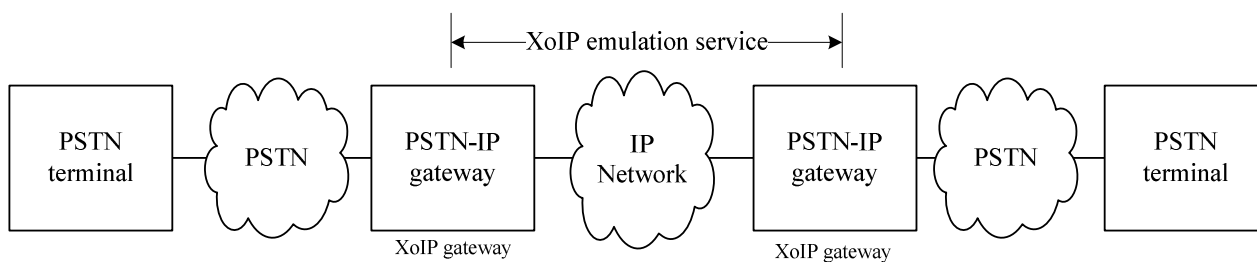
Figure 11: Typical network configuration for PSTN emulation services
