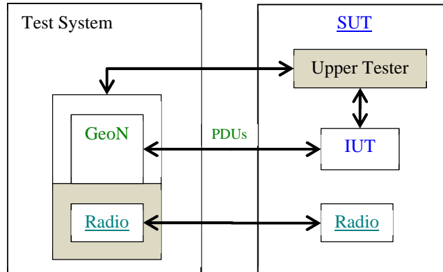
Figure 1: Abstract protocol tester - GeoNetworking
