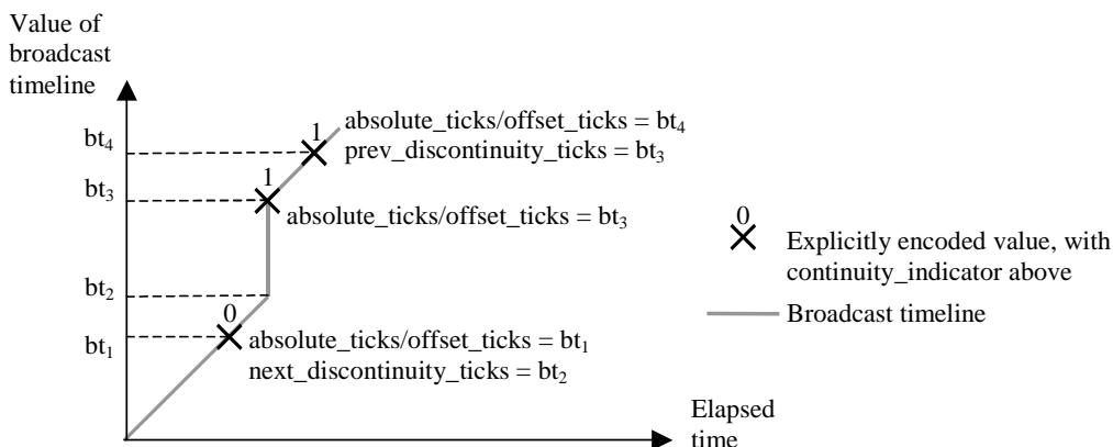
Figure 3: Managing discontinuities in the broadcast timeline
