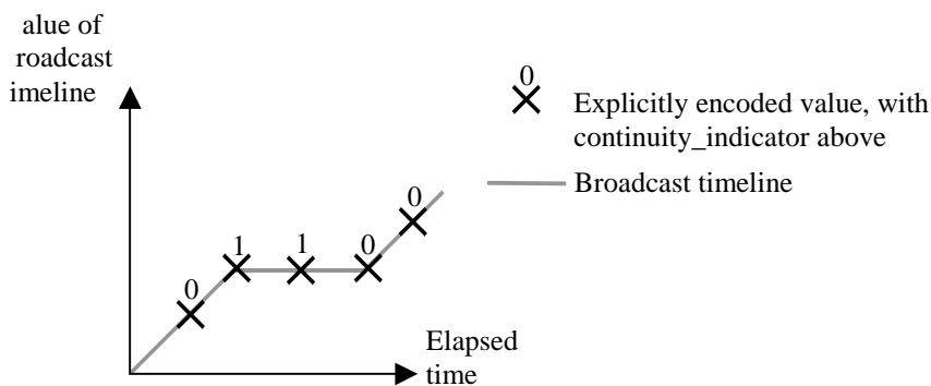
Figure 2: Pausing a broadcast timeline
