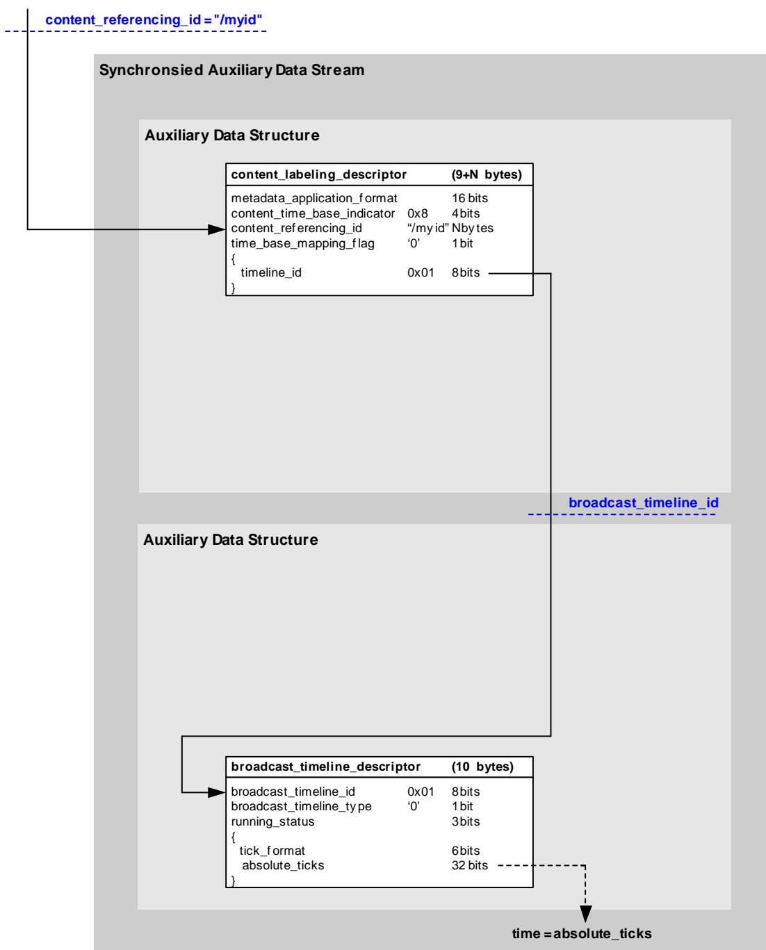
Figure D.3: Implicit linking of broadcast timeline to an item of content
