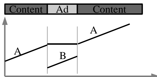
Figure C.2: Advertisement insertion
