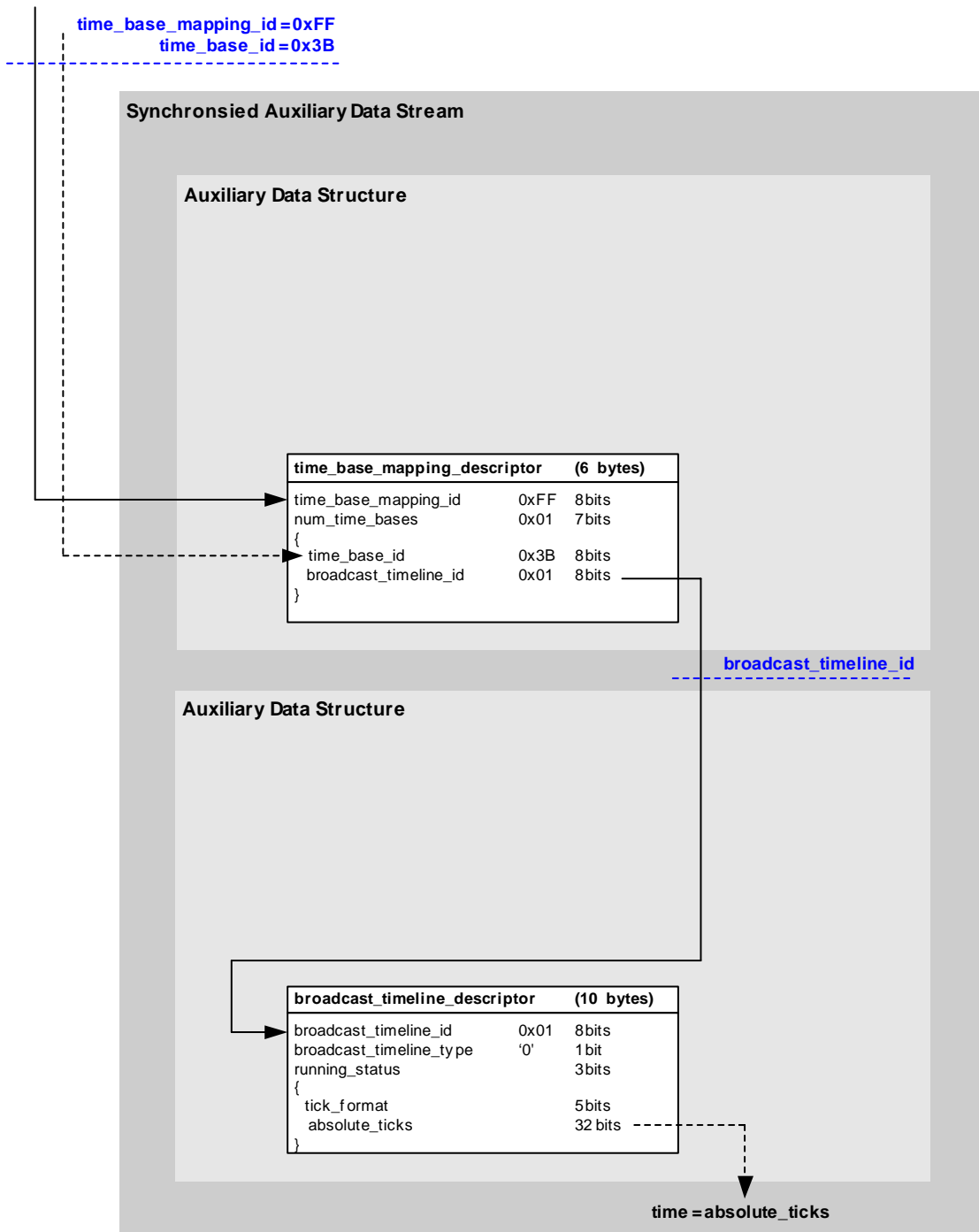
Figure D.5: Independent use of time_base_mapping_descriptor
