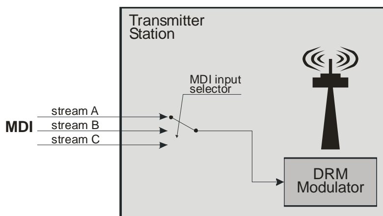
Figure D.1: MDI Switcher setup - local MDI input selection
