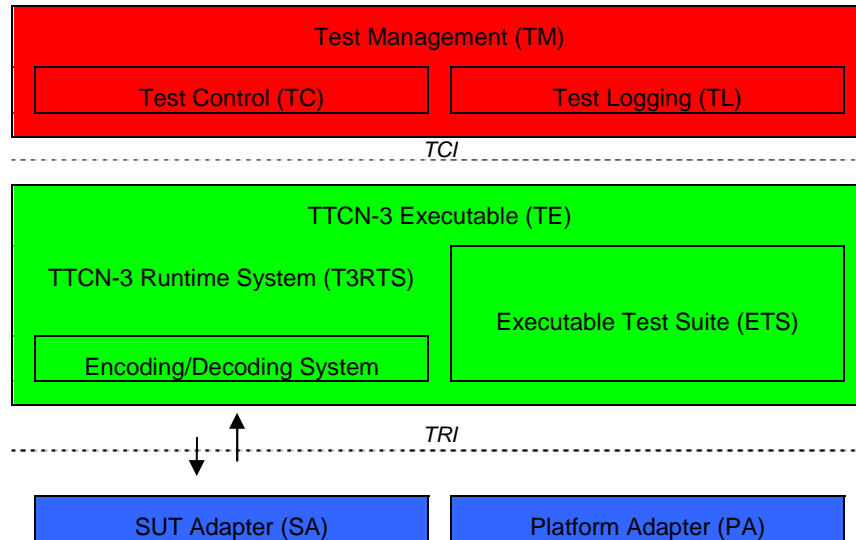
Figure 2: The TTCN-3 Abstract Test System Architecture
