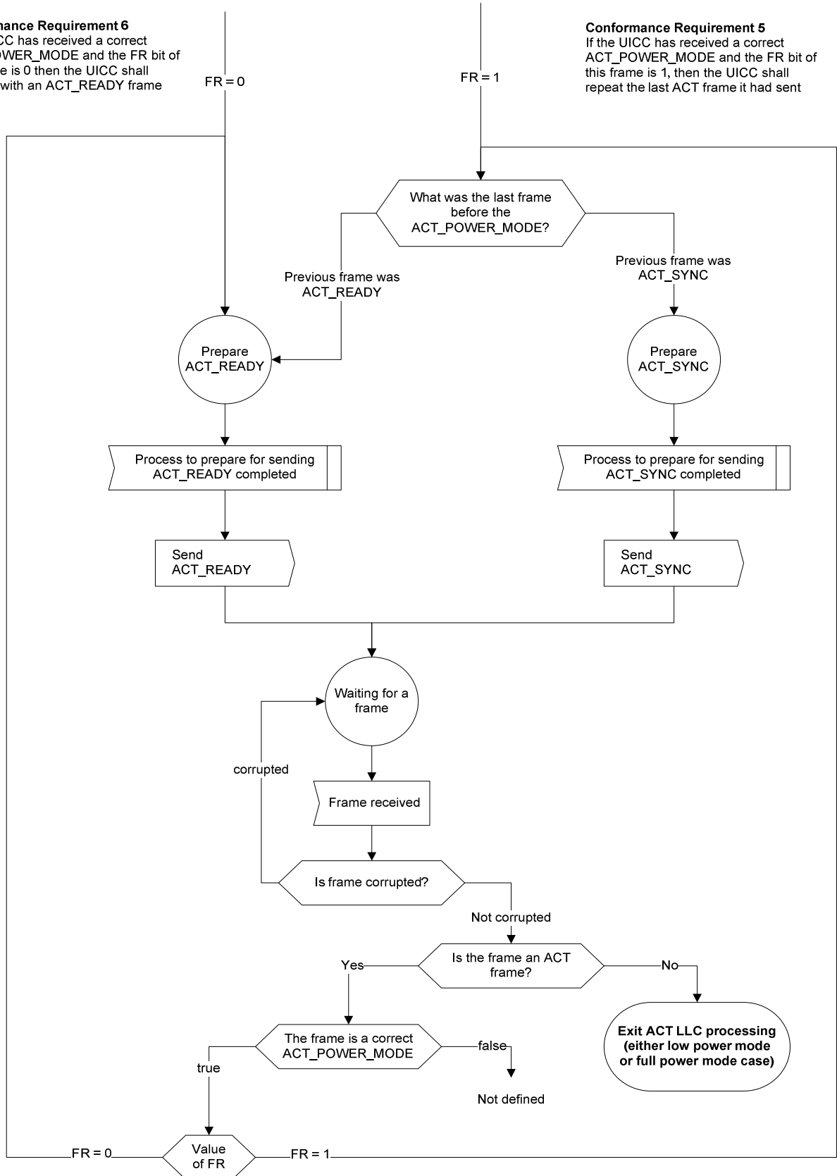
Figure A.2.2: Initial SWP interface activation, part 2
