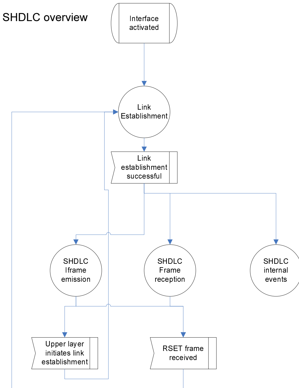
Figure A.3.1: SHDLC overview
