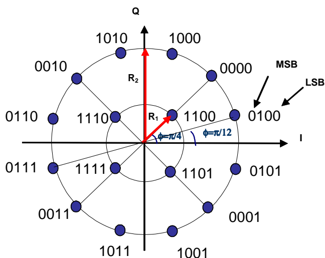
Figure 8: 16APSK modulation
