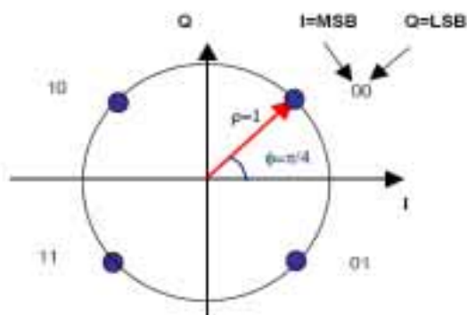
Figure 6: QPSK modulation
