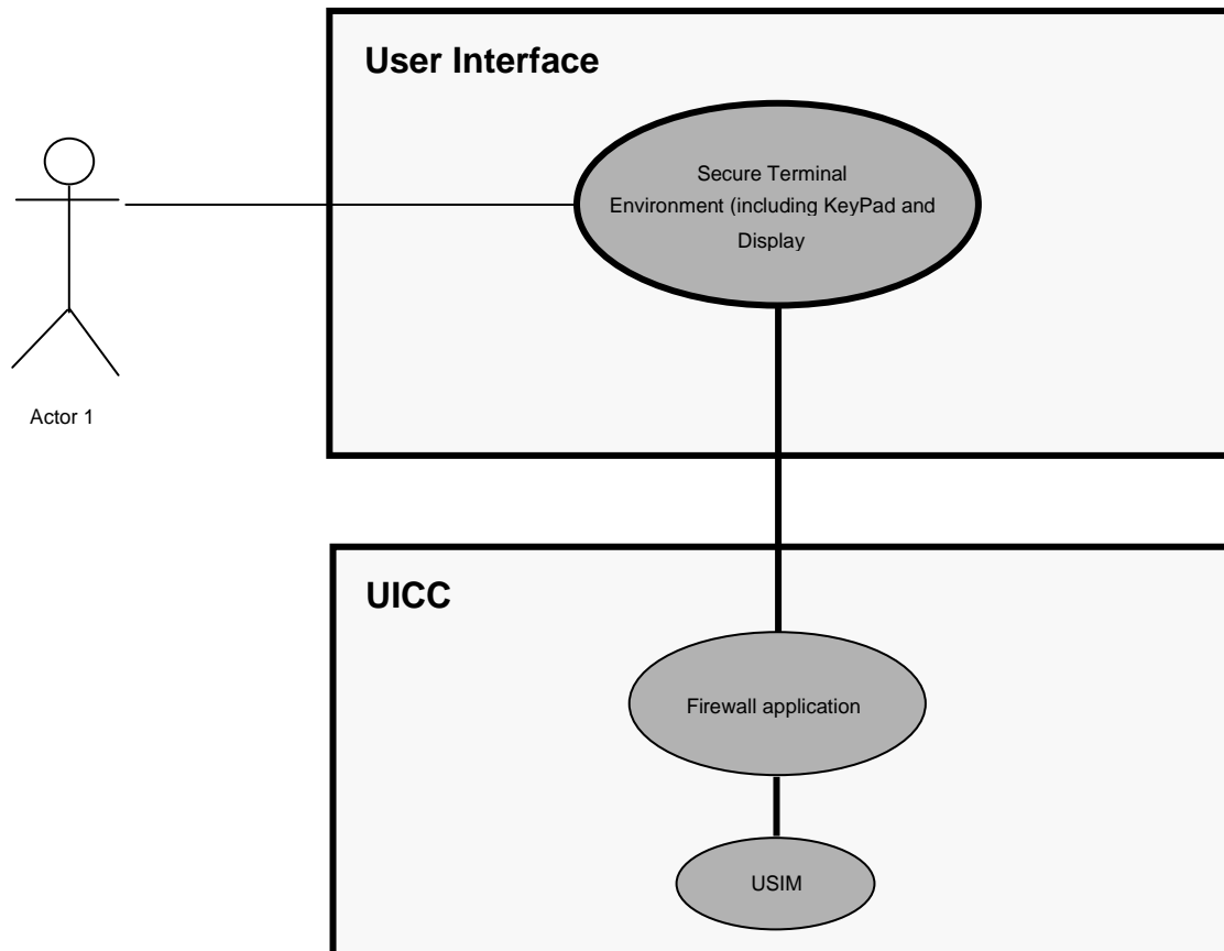
Figure 2: User Interfaces
