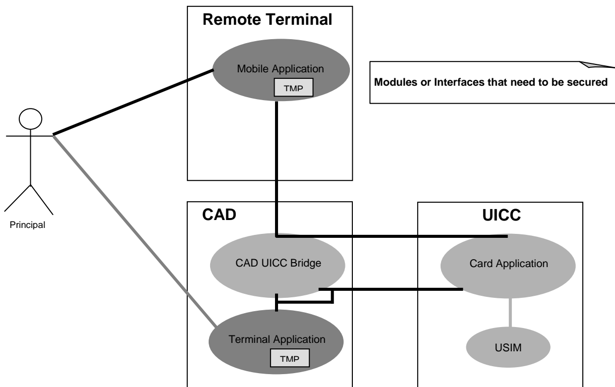
Figure 4: Distributed application
