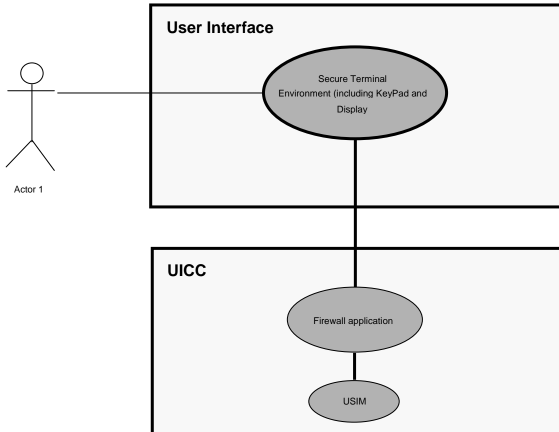
Figure 2: User Interfaces
