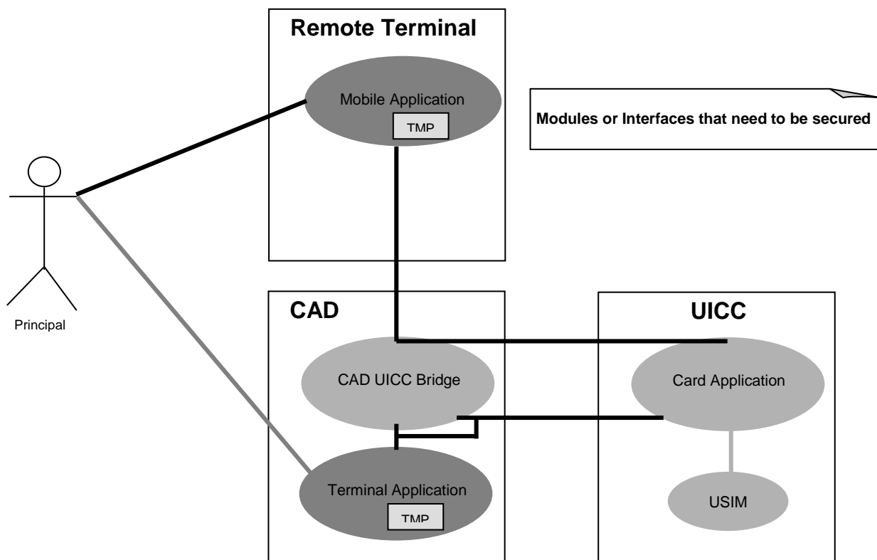
Figure 4: Distributed application
