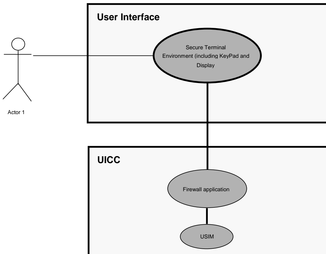
Figure 2: User Interfaces
