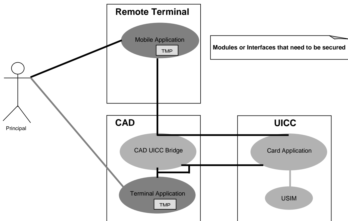
Figure 4: Distributed application
