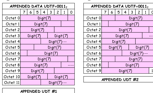
Figure B.12: Unified Data Transport Format (ISO 7 bit) 12 text symbols to 25 text symbols
