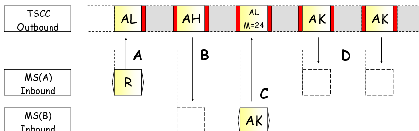
Figure 6.49: Example of the Status Delivery Service to an individual MS
