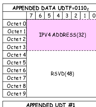
Figure B.22: Appended Data IPV4 format
