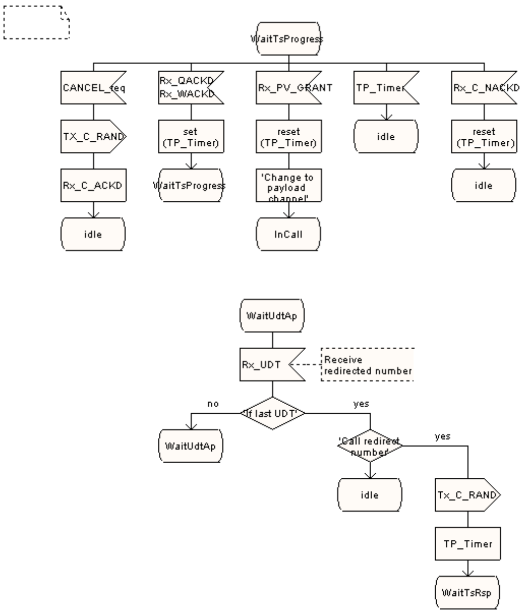
Figure 6.41 (sheet 2 of 2): Single part OACSU voice call setup SDL
