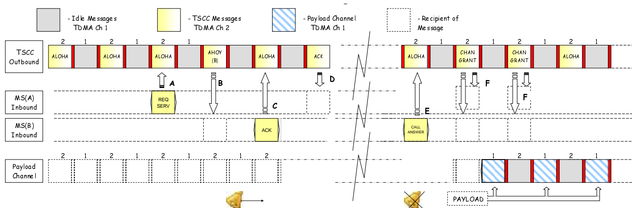
Figure 6.39: Call Answer Mechanism for FOACSU
