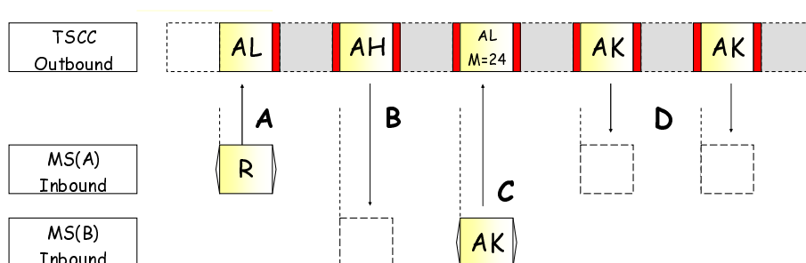
Figure 6.51: Example of the Status Polling Service
