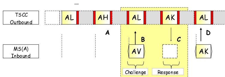
Figure 6.28: MS Kill (with Authentication)
