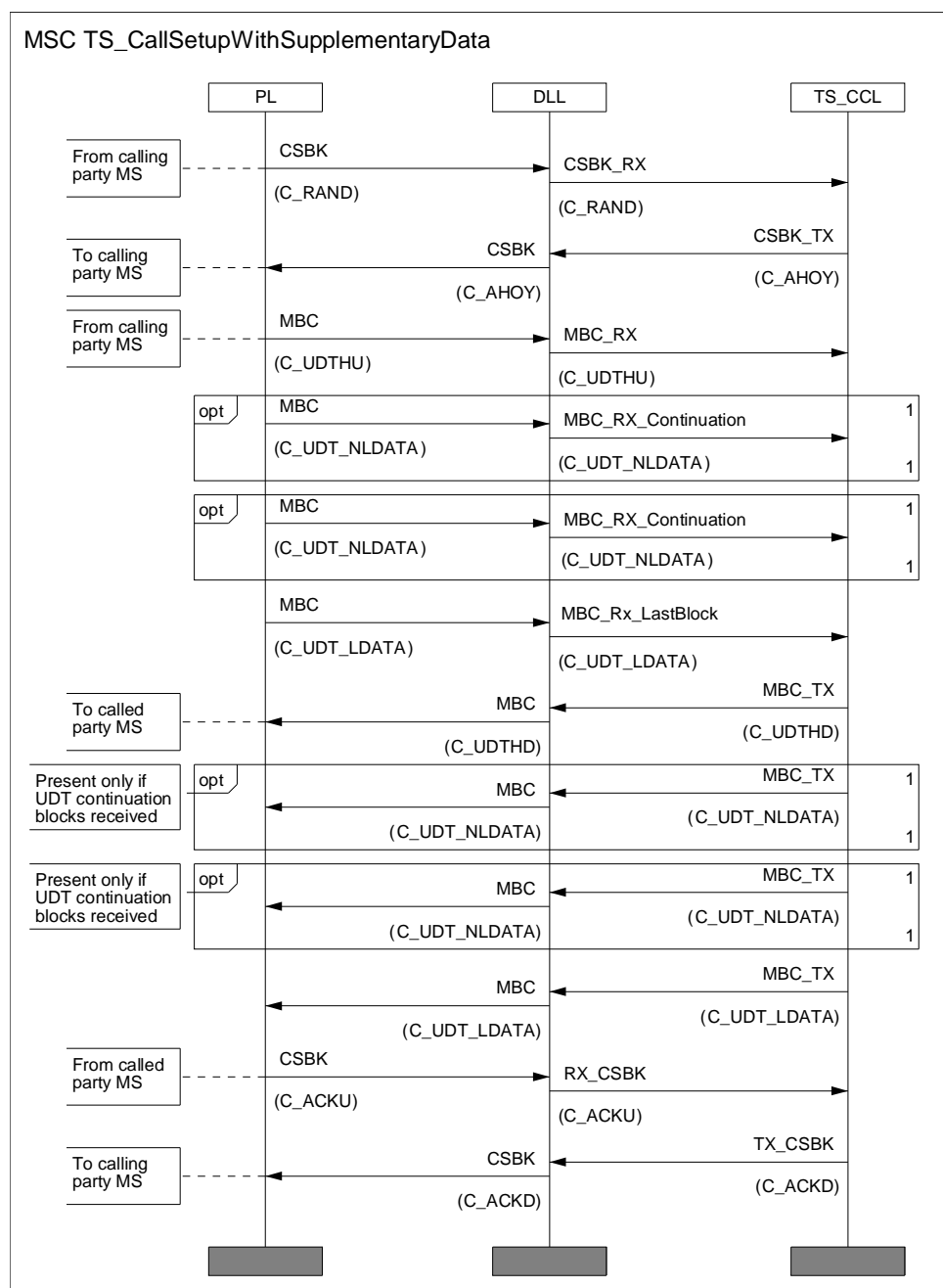
Figure 6.42: MS OACSU Call set-up with Supplementary data
