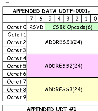
Figure B.6: Appended data Address Format
