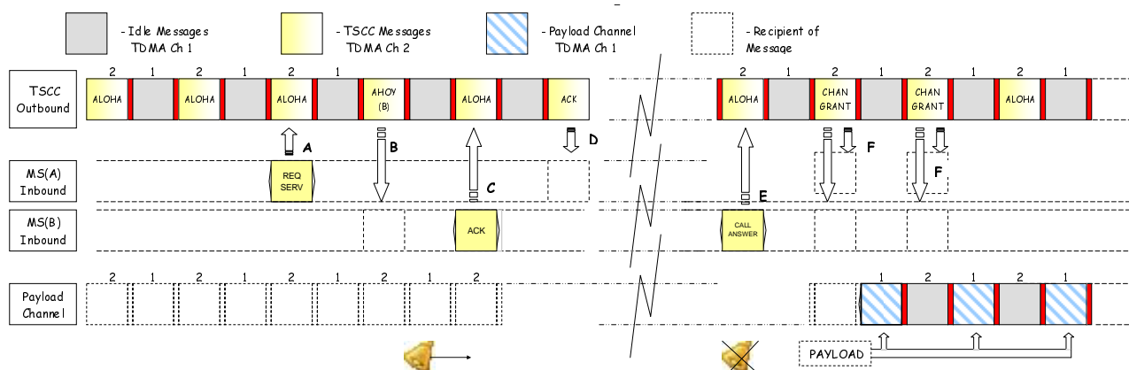
Figure 4.4: Individual Call Set-up example using FOACSU
