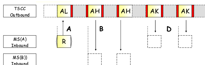
Figure 6.50: Example of the Status Delivery Service to a talkgroup
