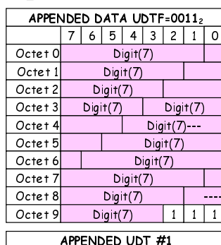
Figure B.11: Unified Data Transport Format (ISO 7 bit) 1 text symbol to 11 text symbols
