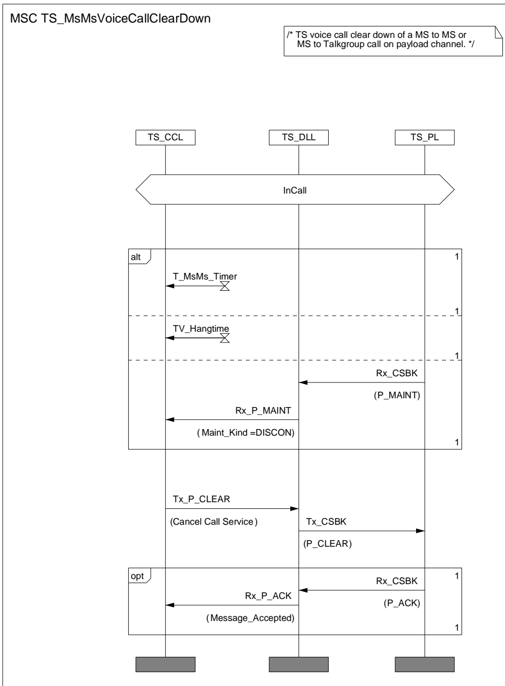
Figure 6.43: Voice Call Termination MSC
