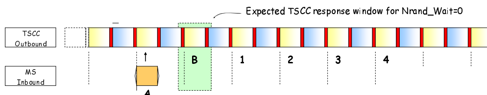
Figure 6.6: Random Backoff Example #1
