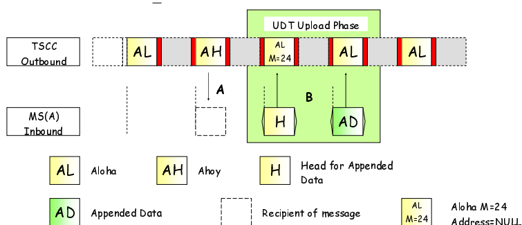
Figure 6.48: Example of UDT short data polling from a gateway
