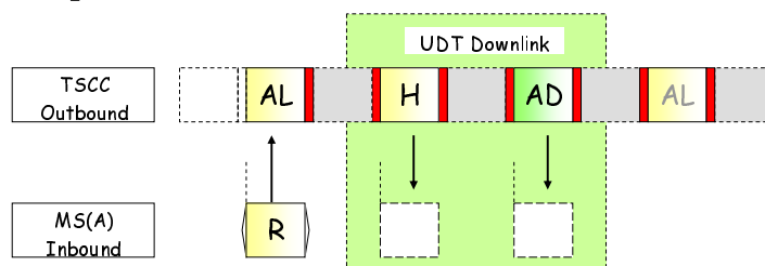
Figure 6.53: TSCC provides diverted address to MS
