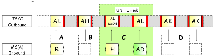
Figure 6.52: Example of a Call Diversion Call
