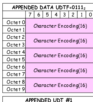
Figure B.24: Unified Data Transport Format (16 bit character) 1 character symbol to 5 character symbols
