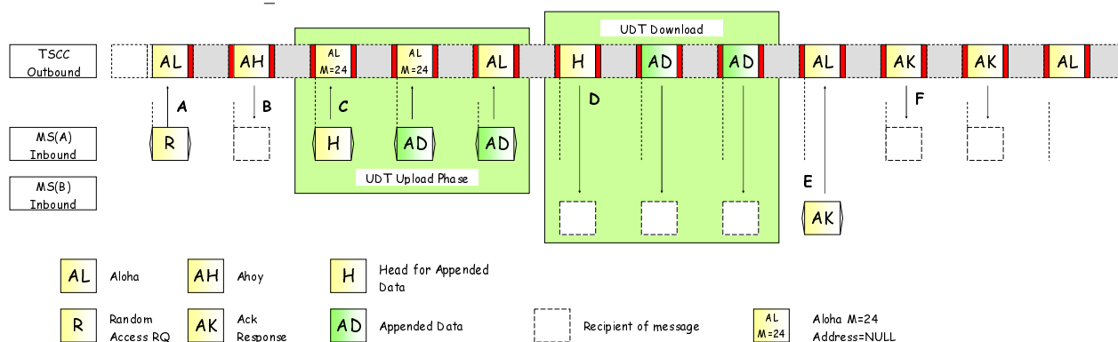
Figure 6.44: Example of a Short Data Message transfer
