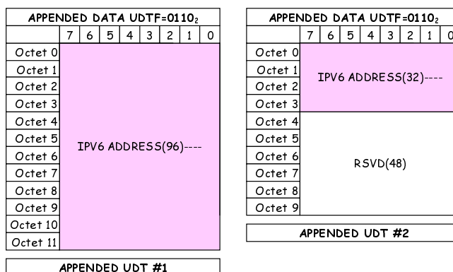
Figure B.23: Appended Data IPv6 format
