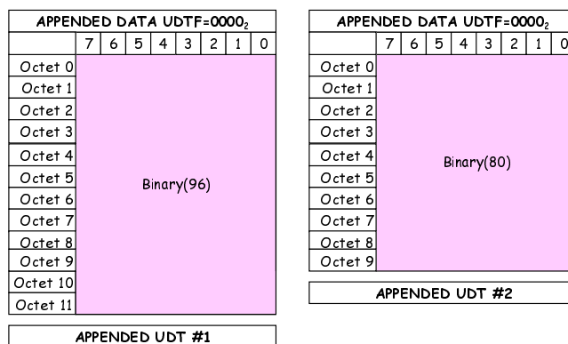
Figure B.3: Unified Data Transport Format (Binary) 80 bits to 175 bits
