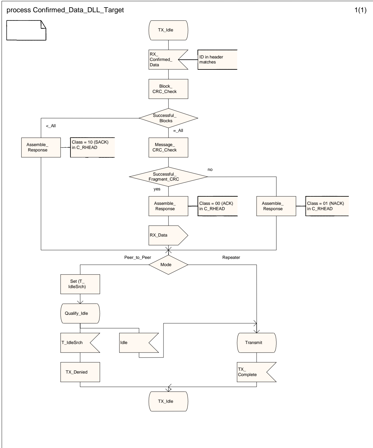
Figure 5.9: Target Confirmed Data Transmission SDL
