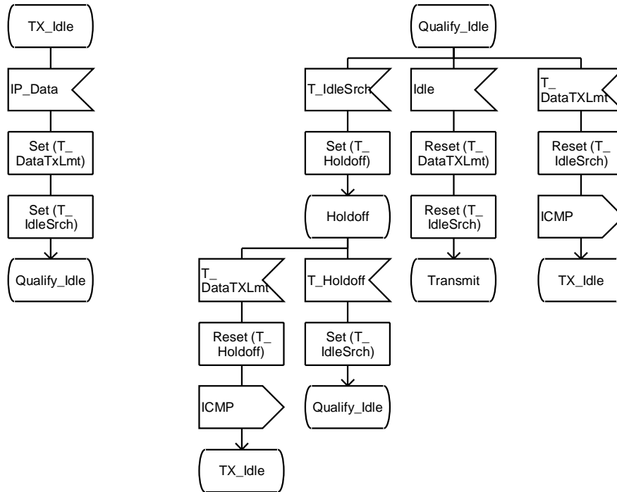
Figure 5.4: Unconfirmed IP Data Channel Access SDL
