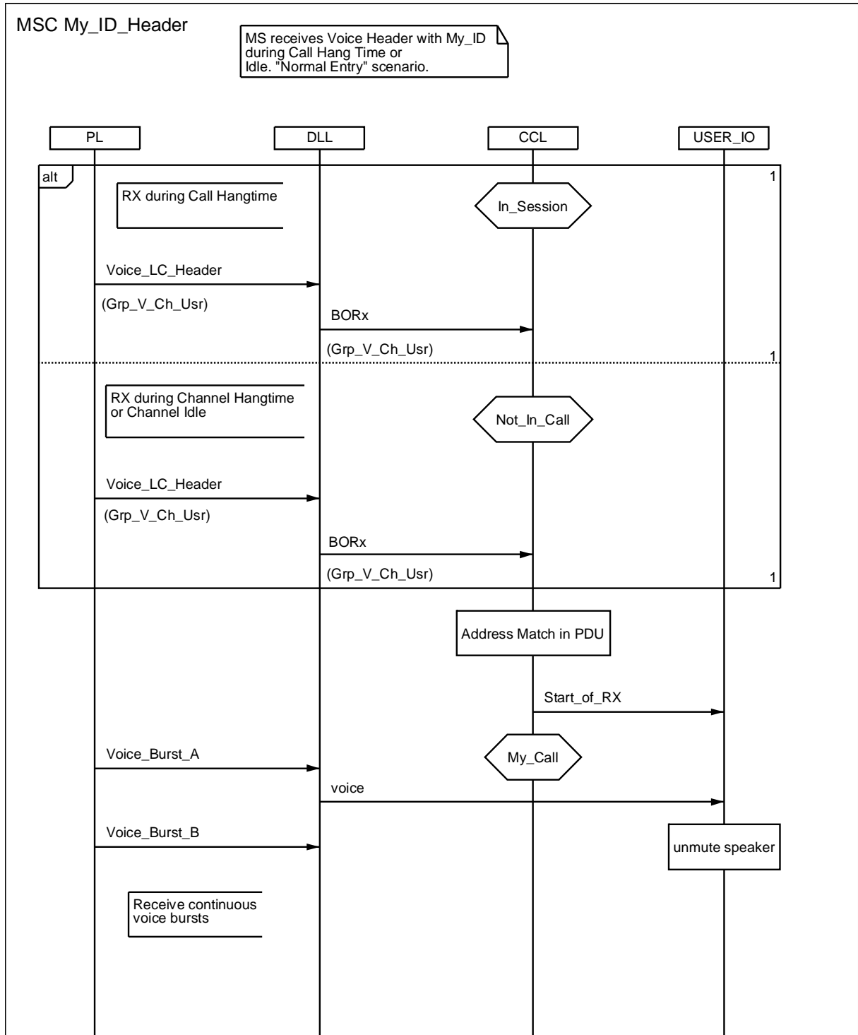
Figure 5.15: MSC My_Header_LC
