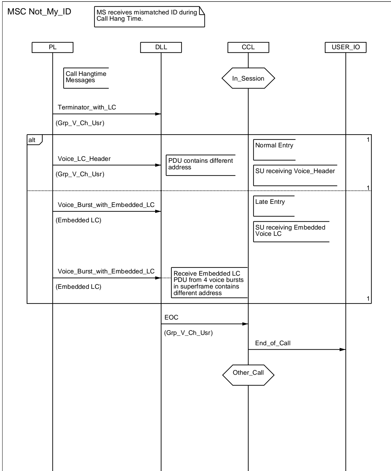
Figure 5.20: MSC Not_My_ID
