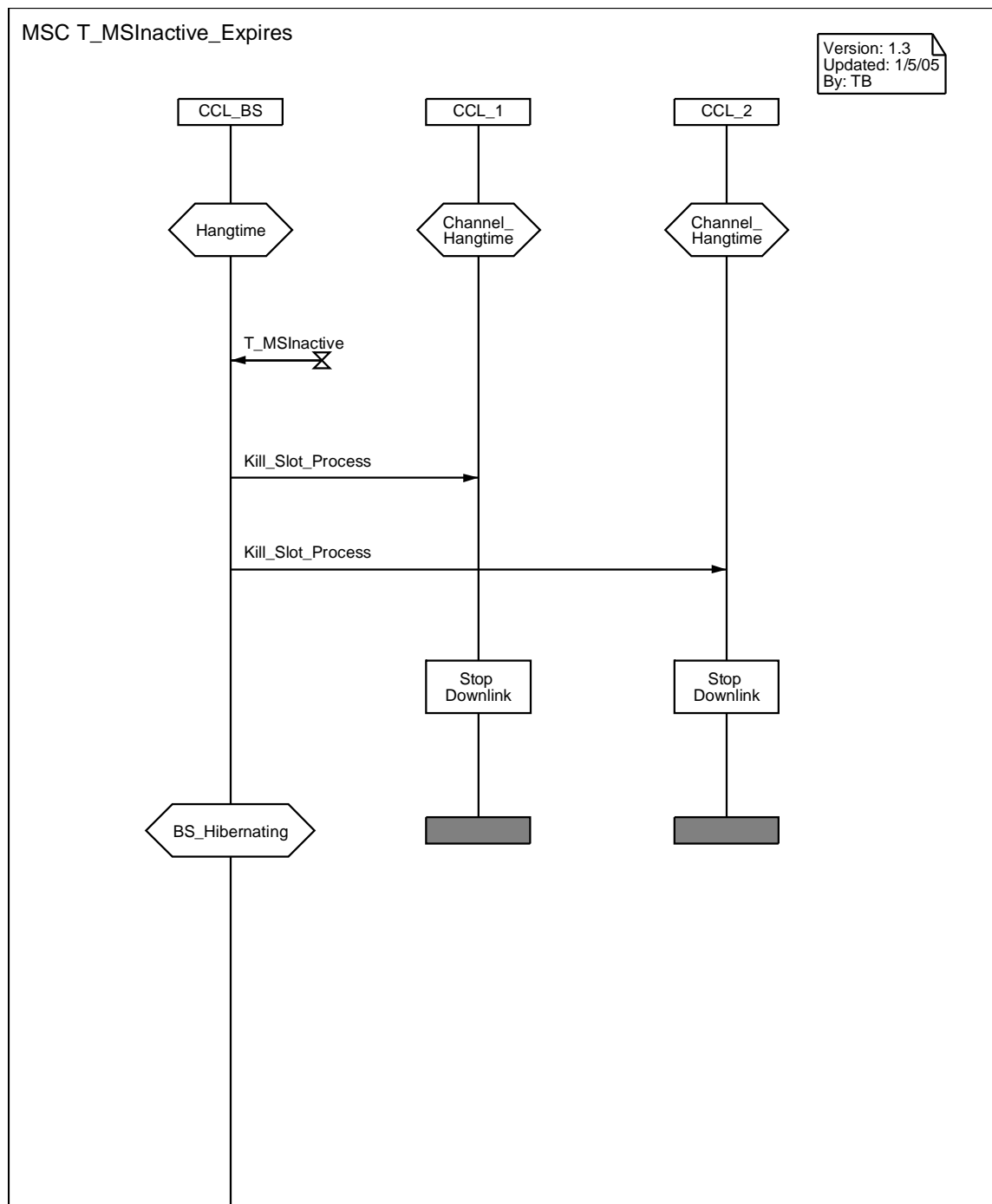
Figure 5.8: BS_Outbound_Deactivation
