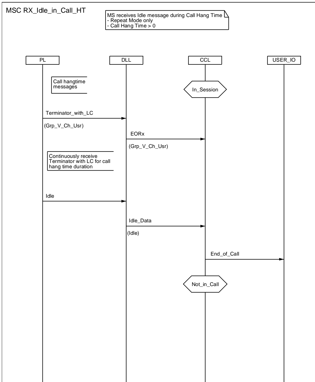
Figure 5.19: MSC RX_Idle_SYNC_in_Call_HT
