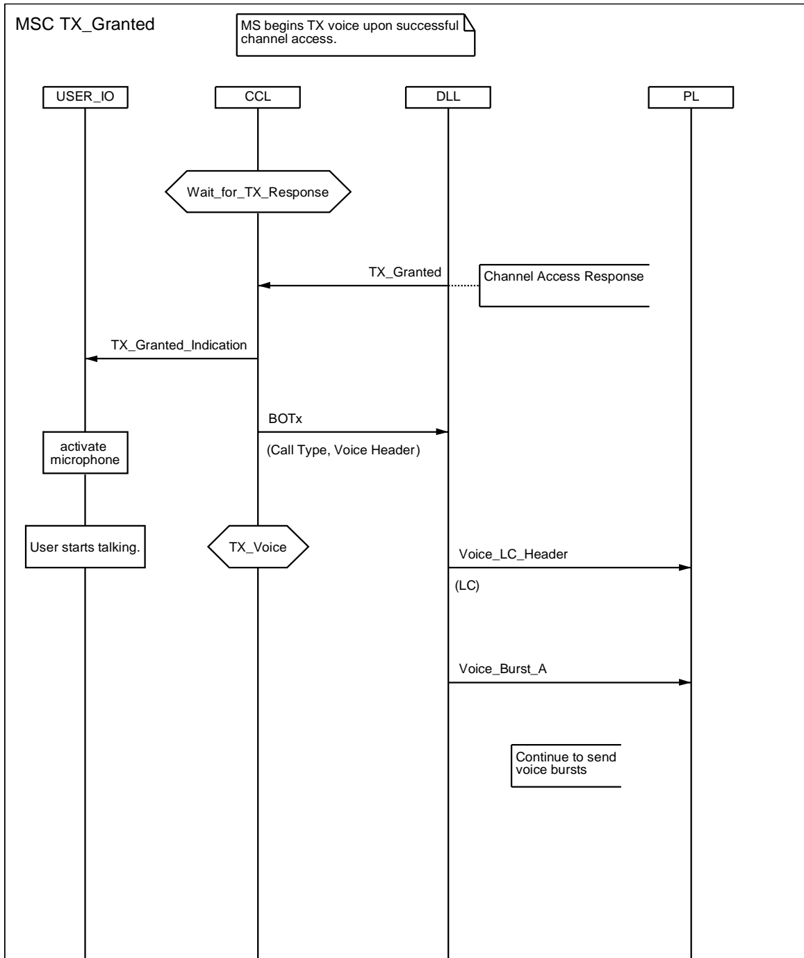
Figure 5.14: MSC TX_Granted
