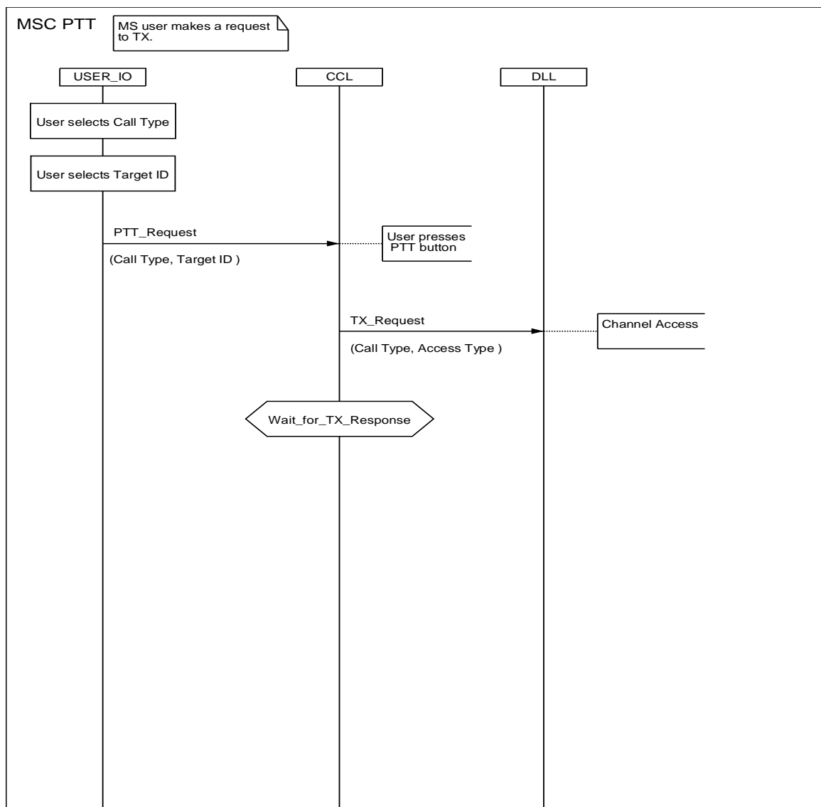
Figure 5.12: MSC PTT
