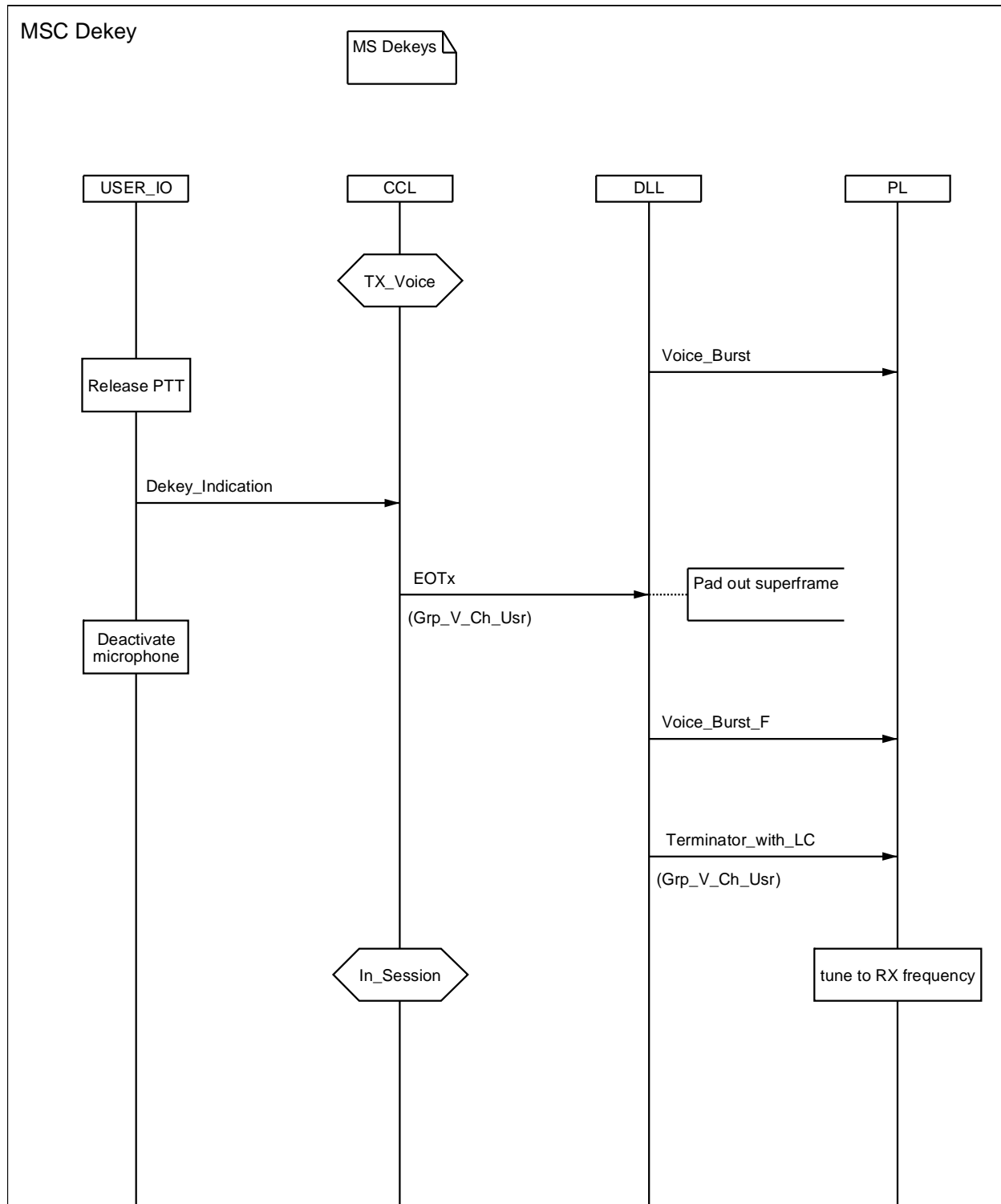
Figure 5.17: MSC Dekey
