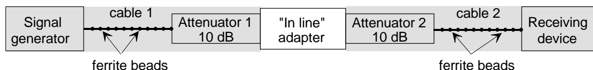
Figure 27: Stage 1: Direct attenuation measurement for the verification procedure
