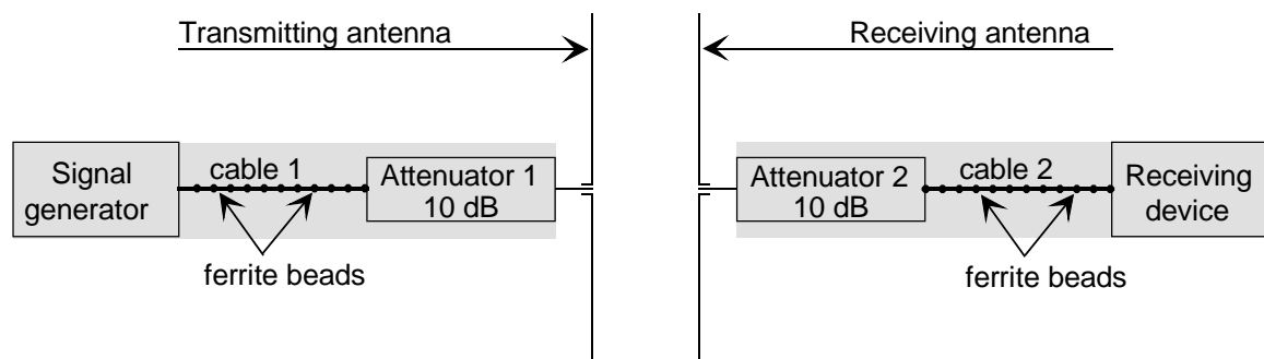
Figure 23: Stage 2: NSA measurement
