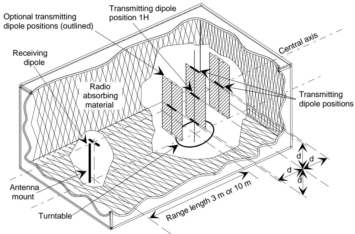
Figure 4: Antenna arrangements for horizontal polarization
