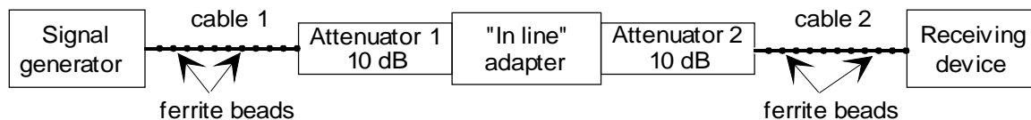
Figure 15: Initial equipment arrangement for the verification tests
