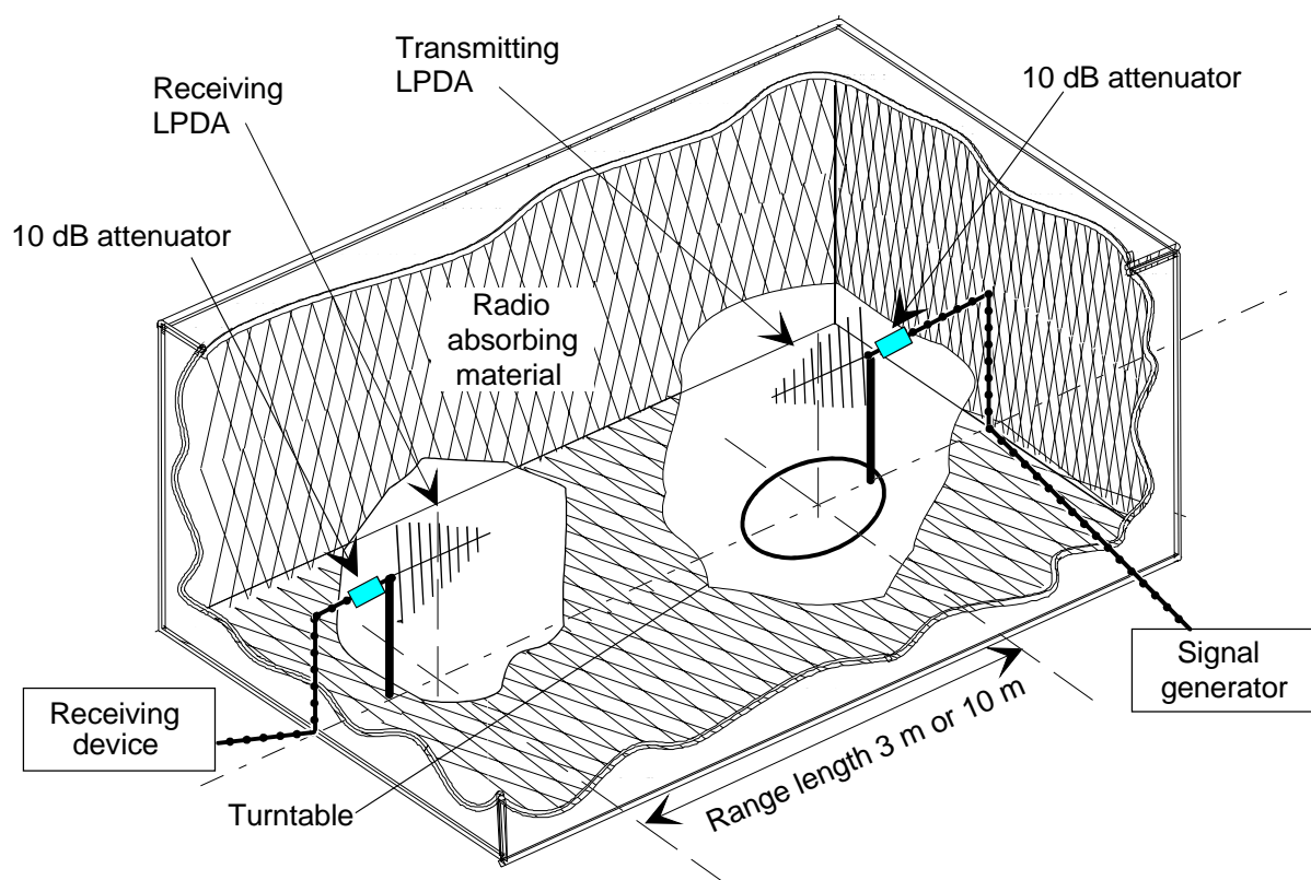
Figure 14: Anechoic chamber layout for verification with LPDAs
