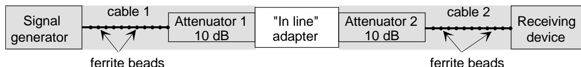
Figure 25: Stage 1: Direct attenuation measurement for the verification procedure
