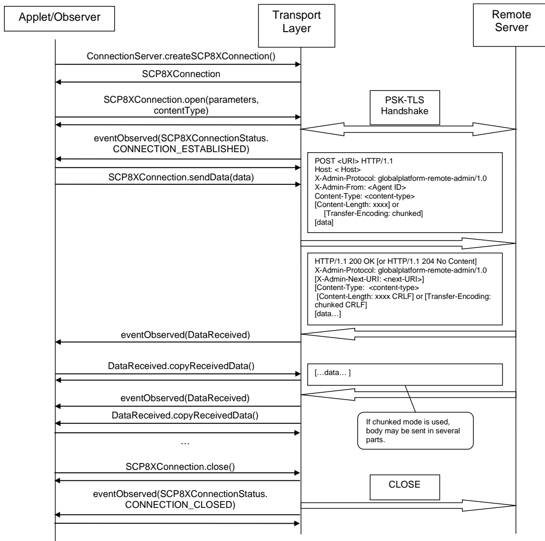
Figure 5: SCP8XConnection for SCP81sequence diagram
