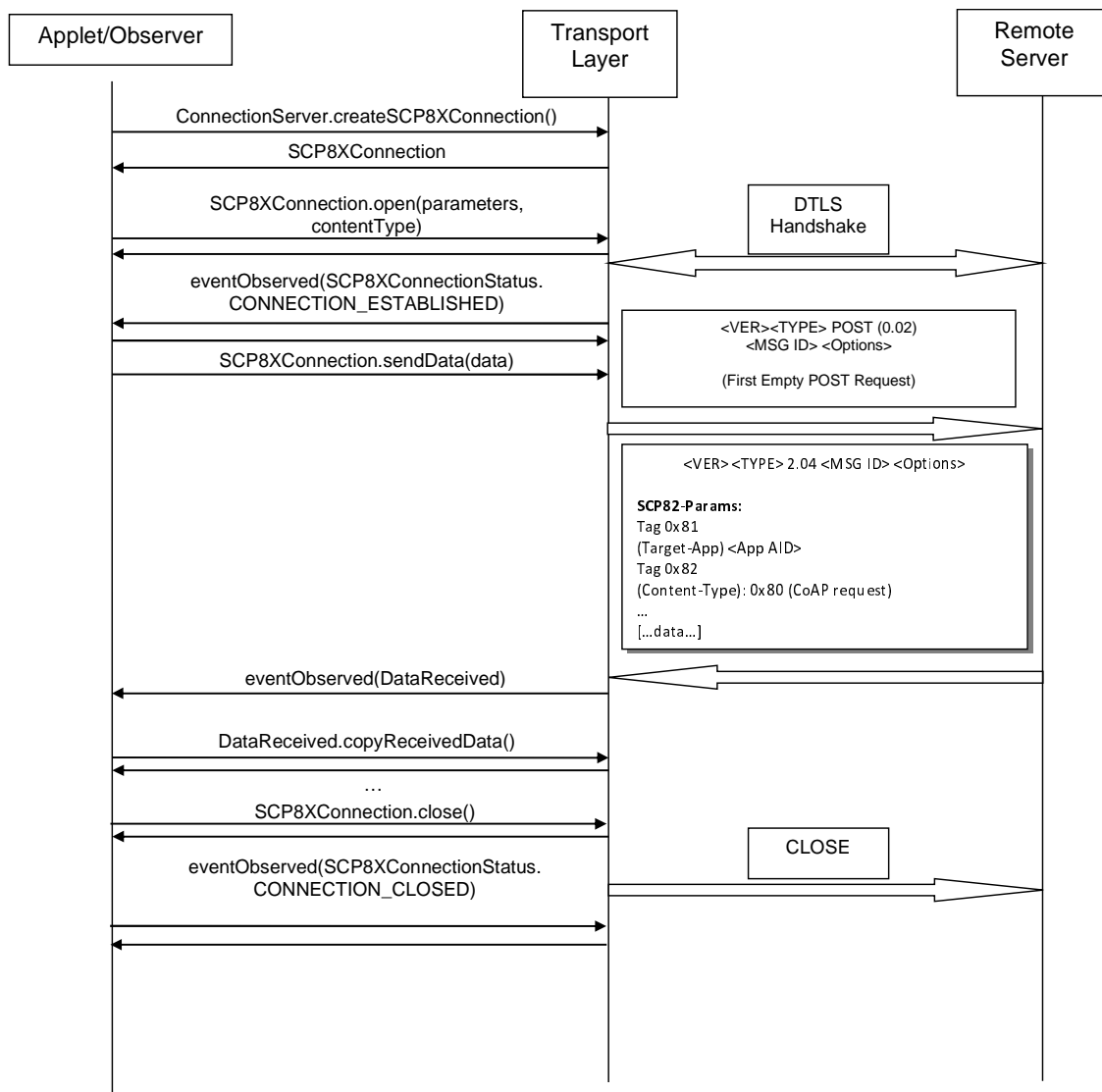
Figure 6: SCP8XConnection for SCP82 sequence diagram
