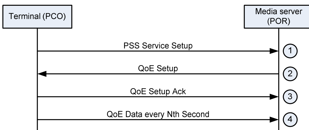
Figure B.2: Media Quality measurement for the 3GPP PSS service
