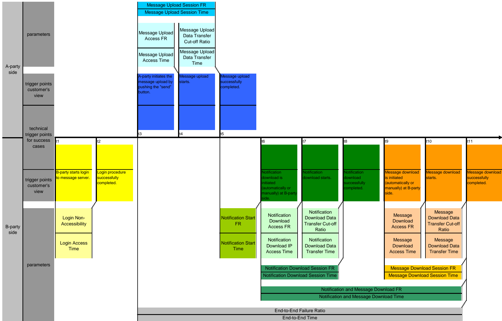
Figure 52: Generic Store-and-forward Parameter Overview
