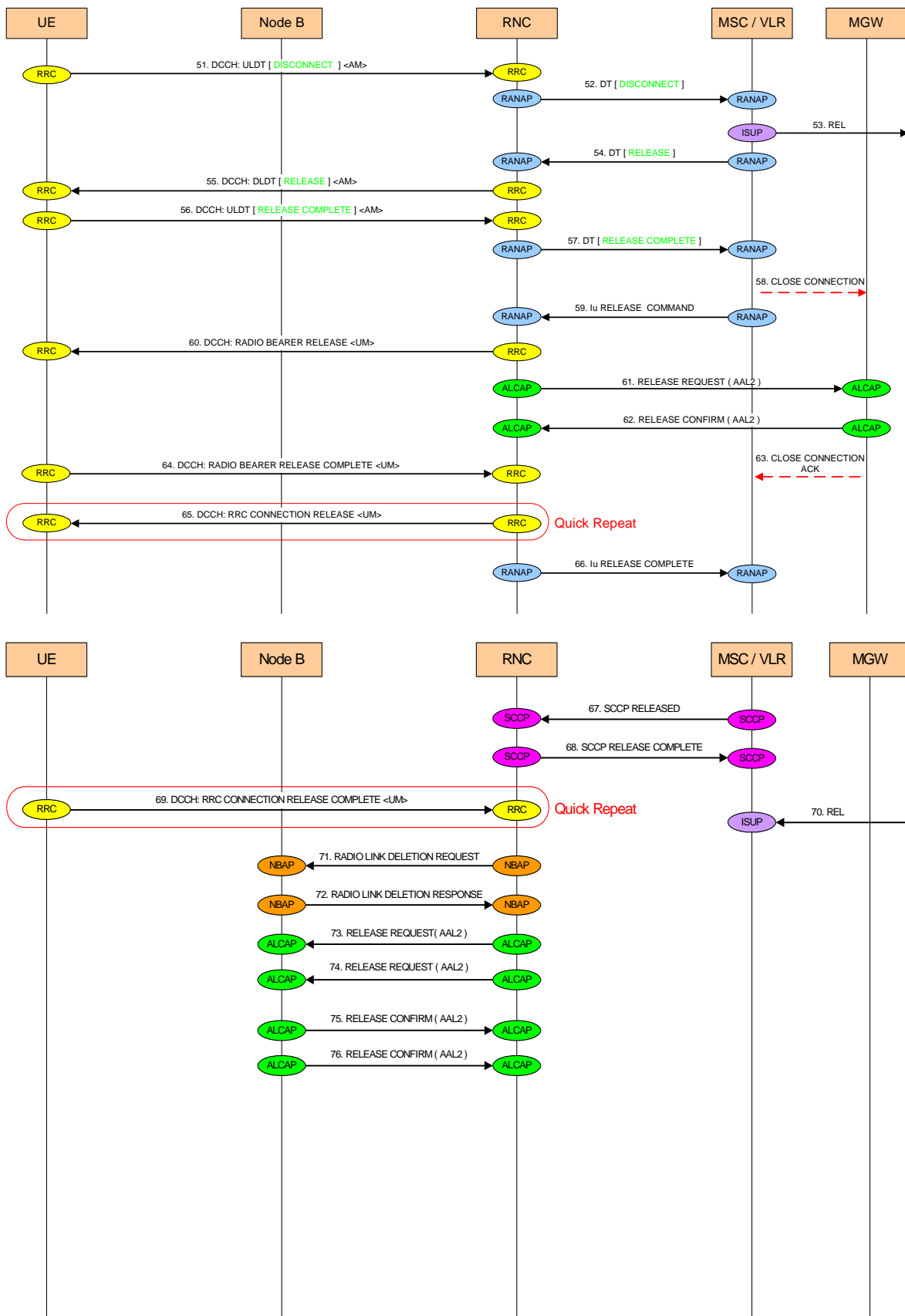
Figure 24: 3G telephony signalling flow chart: mobile initiated call disconnection procedure
