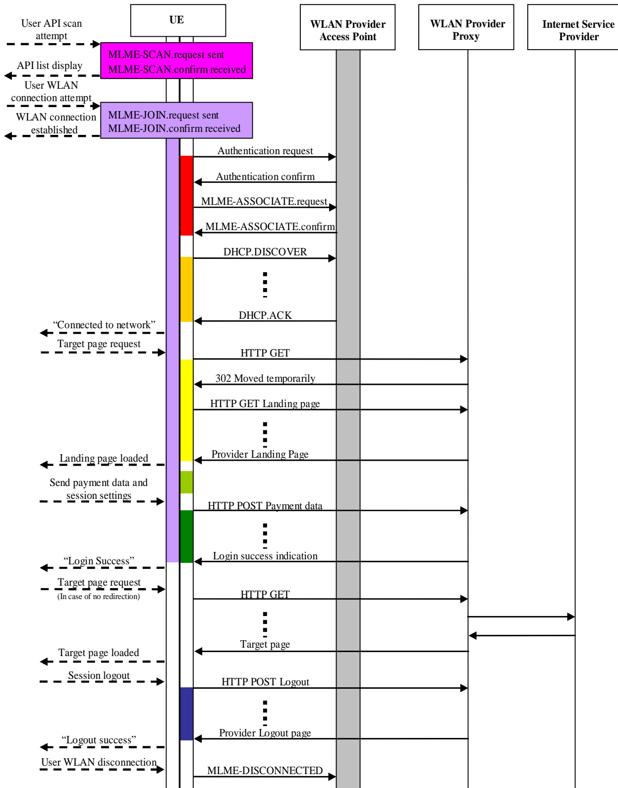
Figure 27: Generic Signal Flow
