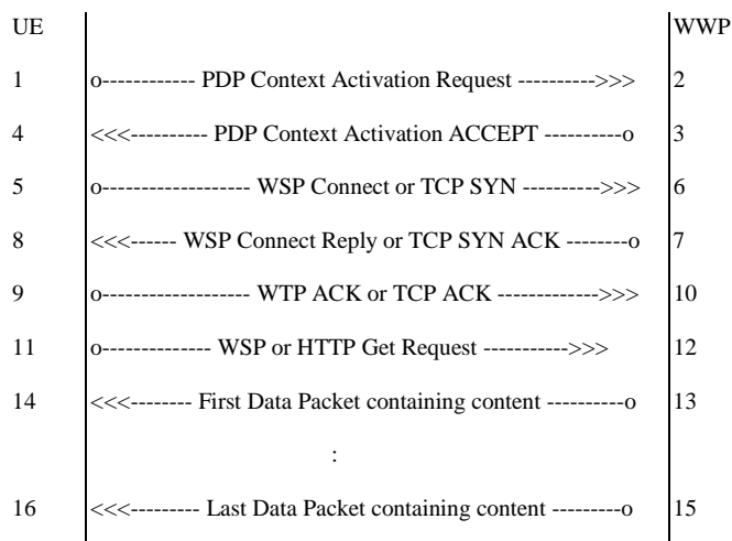
Figure 39: WAP Message Sequence Chart
