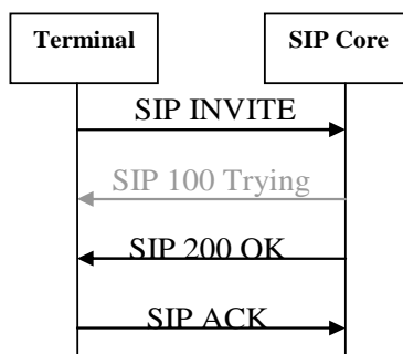
Figure 11: Media parameters negotiation for pre-established session
