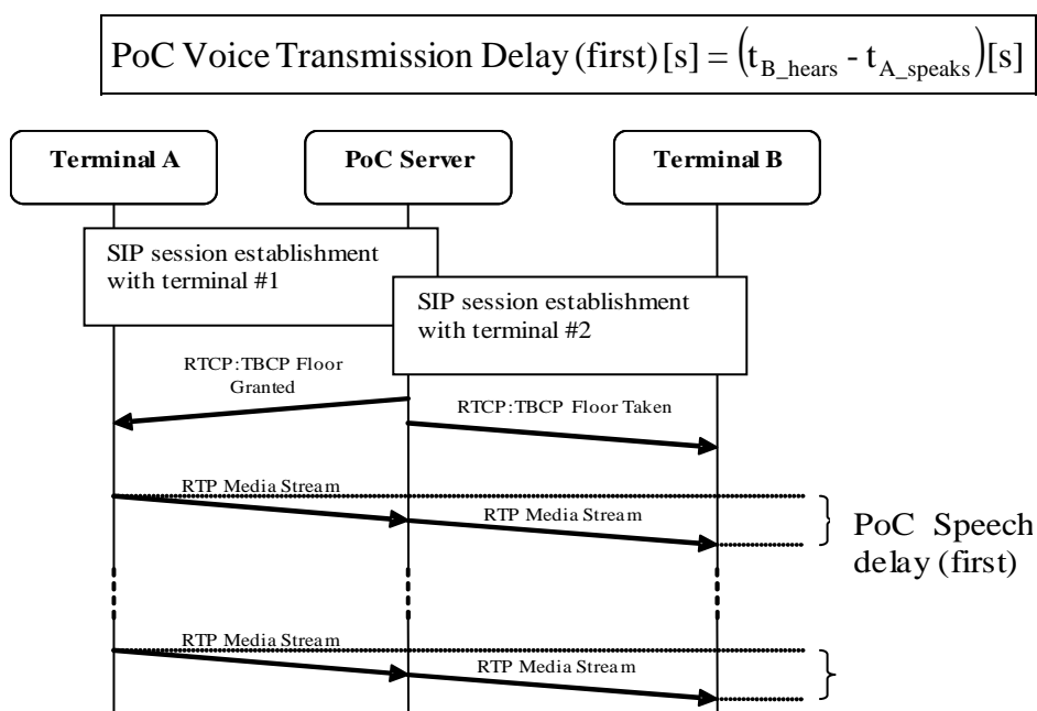
Figure 20: PoC speech transmission delay (first) and PoC speech transmission delay (others)
