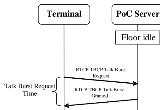
Figure 18: Example for a successful talk burst request
