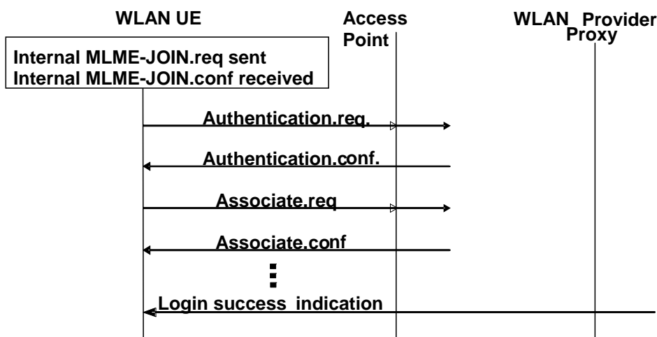
Figure 33: WLAN PS Data Service Provisioning Signal Flow
