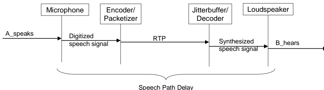
Figure 46: The Speech Path Delay
