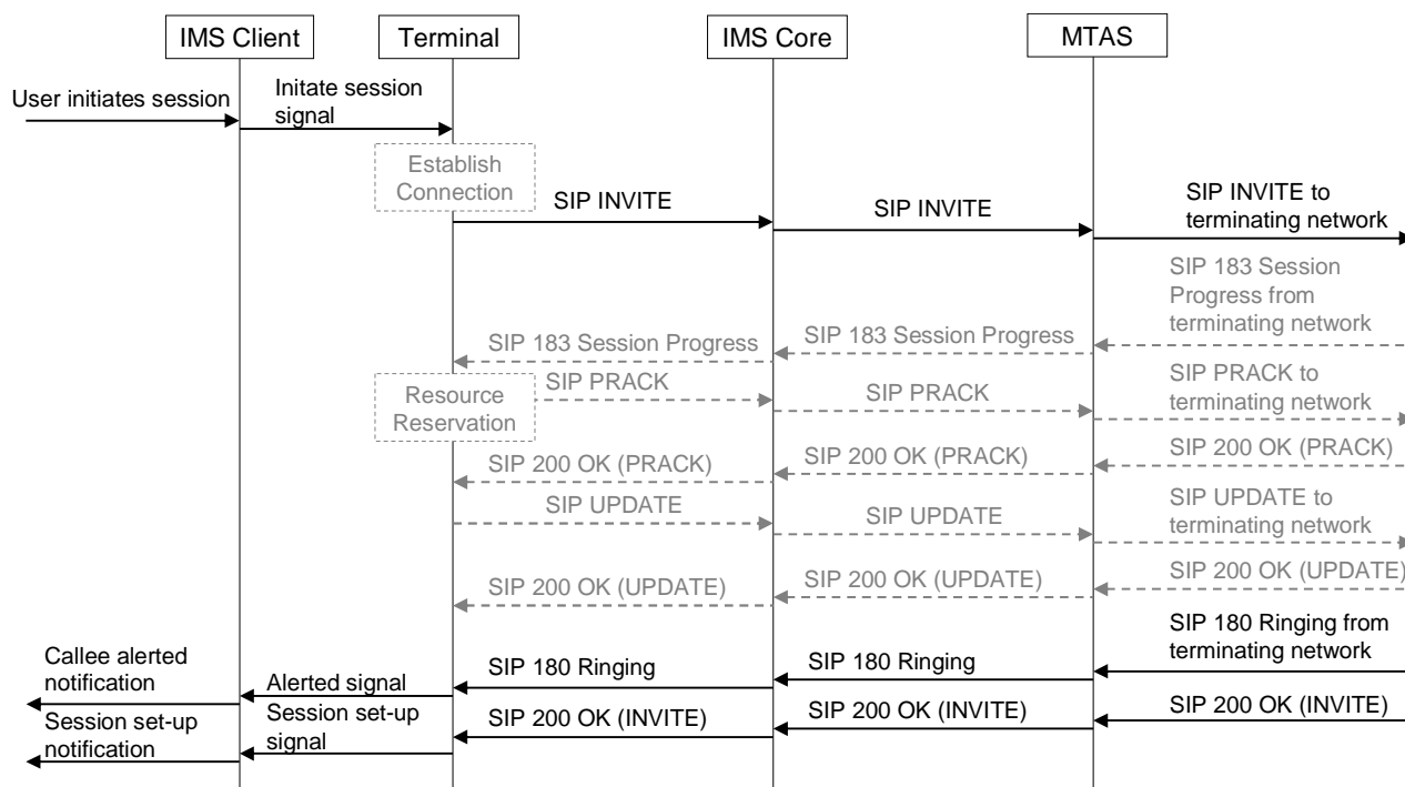
Figure 42: Implicit Initiation of the MTSI Session
