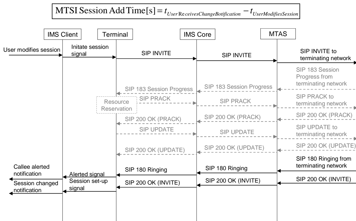
Figure 43: Modification of the MTSI Session
