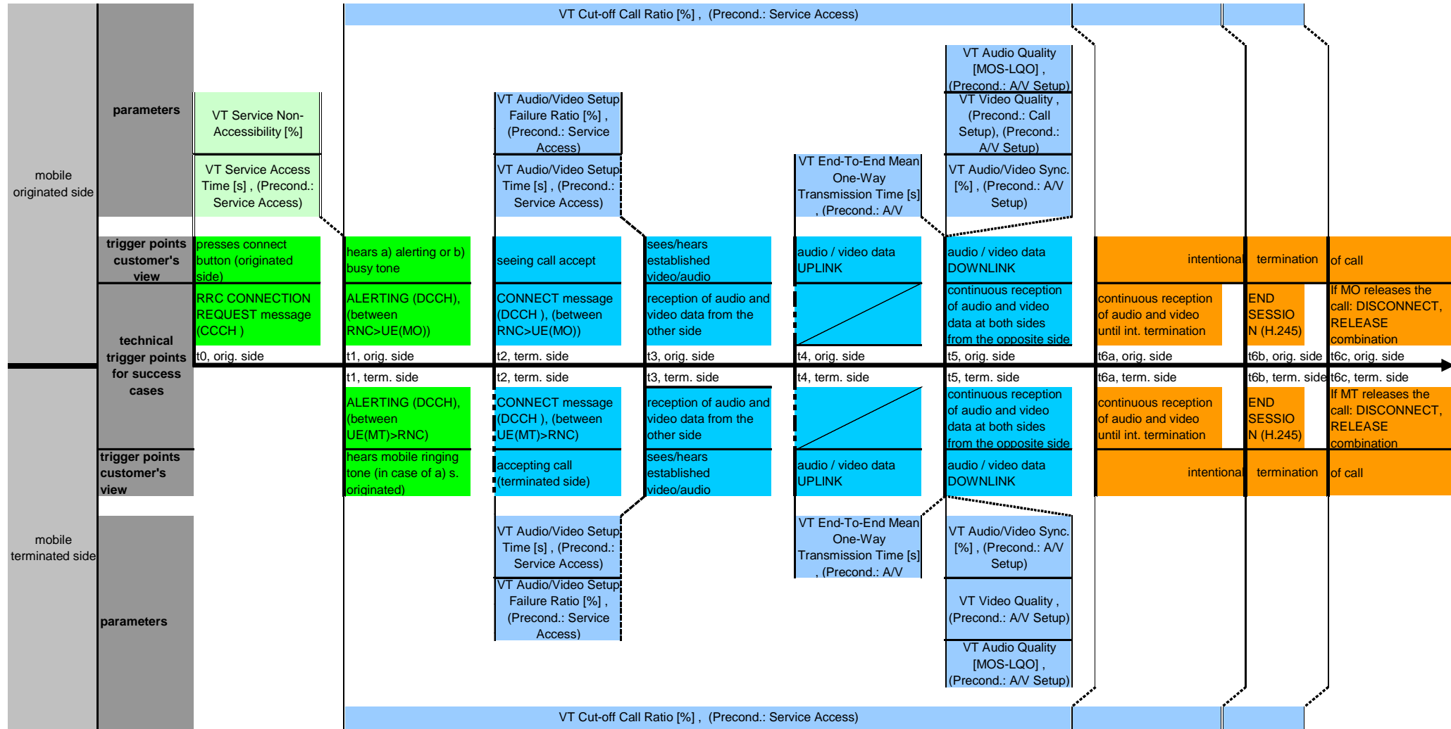
Figure 25: Parameter overview with trigger points
