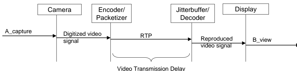
Figure 47: The Video Transmission Delay
