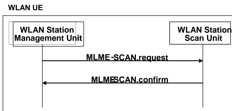
Figure 29: SCAN Signal Flow
