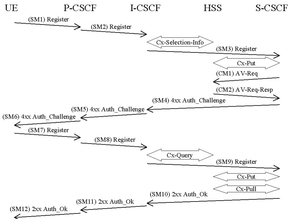
Figure 41: Successful MTSI registration example
