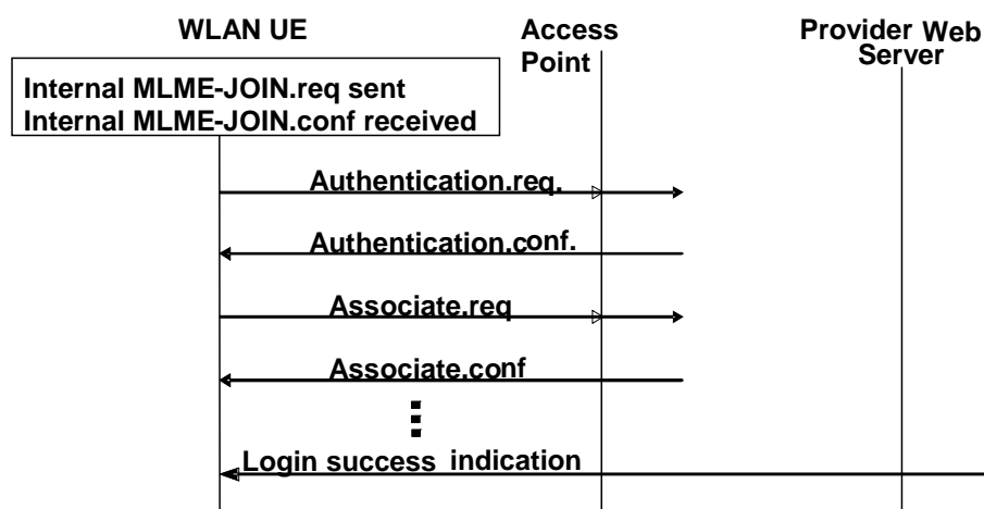
Figure 31: WLAN PS Data Service Provisioning Signal Flow
