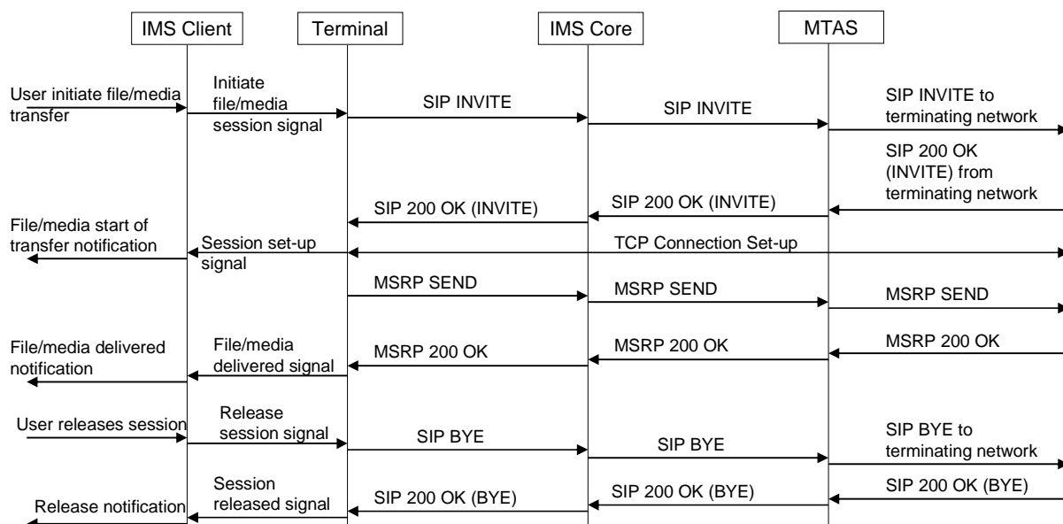
Figure 51: File/Media Sharing using MTSI
