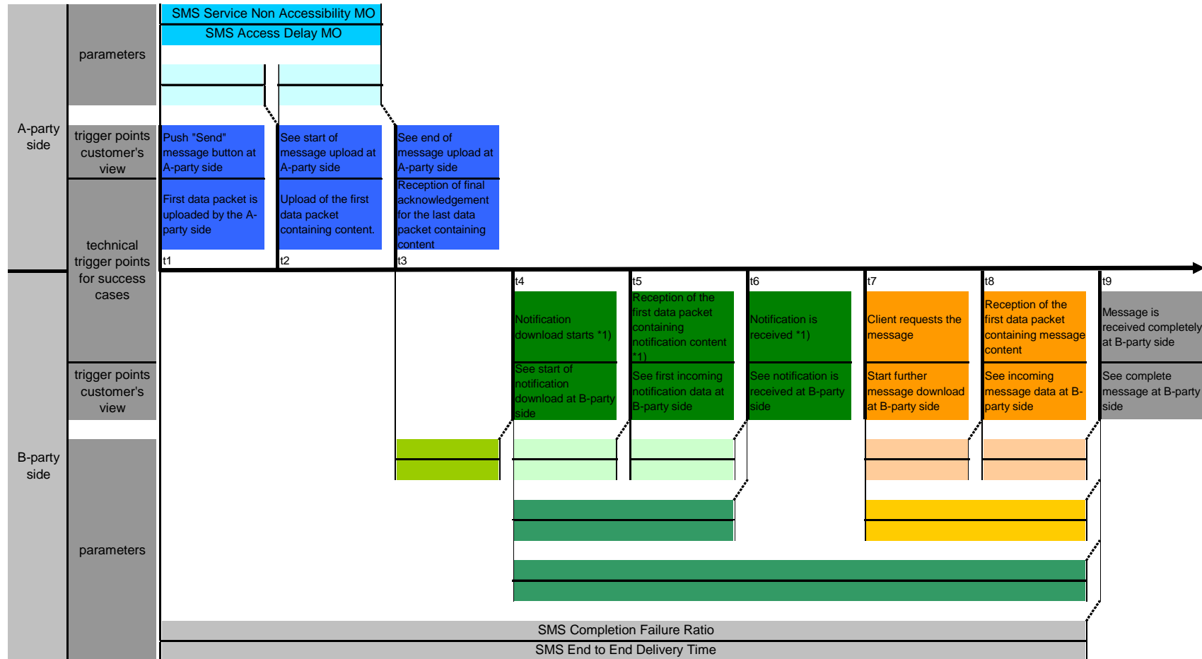
Figure 59: SMS Parameter Overview with Trigger Points
