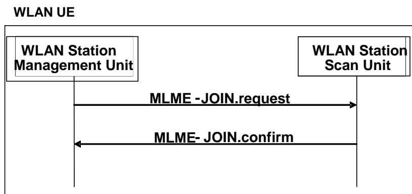
Figure 32: JOIN Signal Flow
