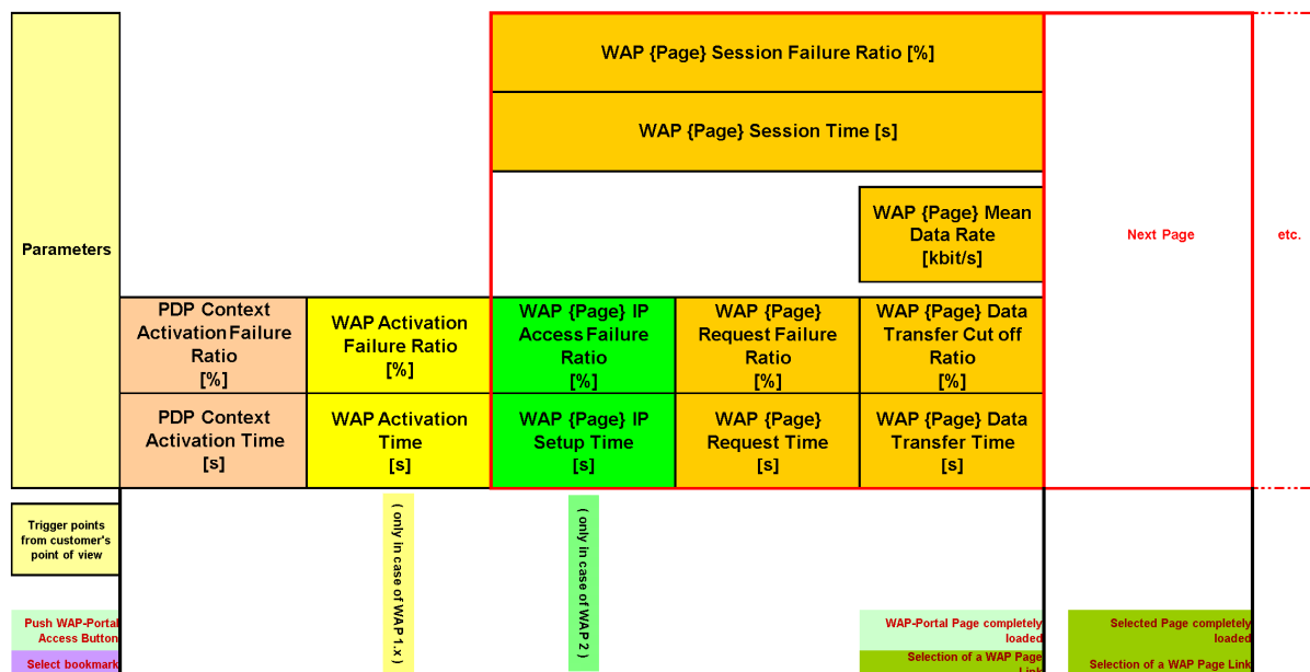
Figure 38: Parameter and service overview
