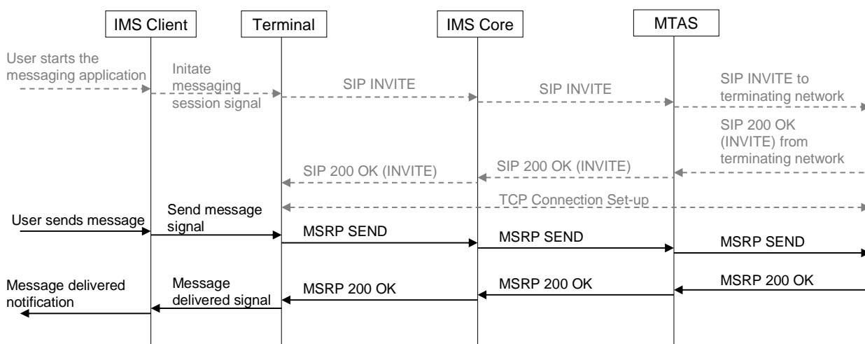
Figure 50: Messaging using MSRP
