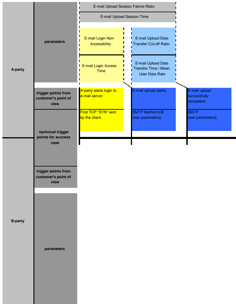
Figure 54: SMTP Overview
