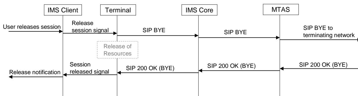
Figure 44: Signalling to end an MTSI Session
