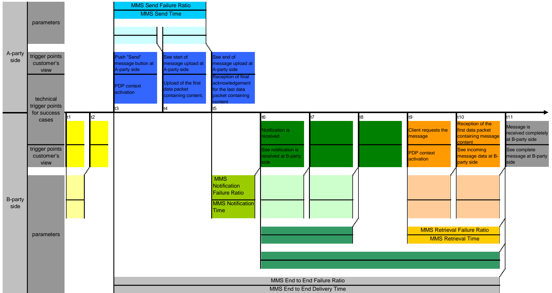
Figure 57: MMS Parameter Overview with Trigger Points
