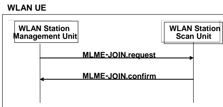
Figure 30: JOIN Signal Flow
