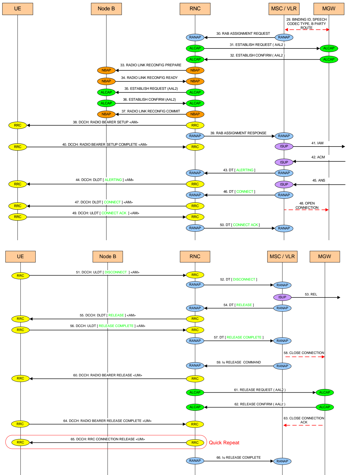
Figure 26: Video telephony signalling flow chart
