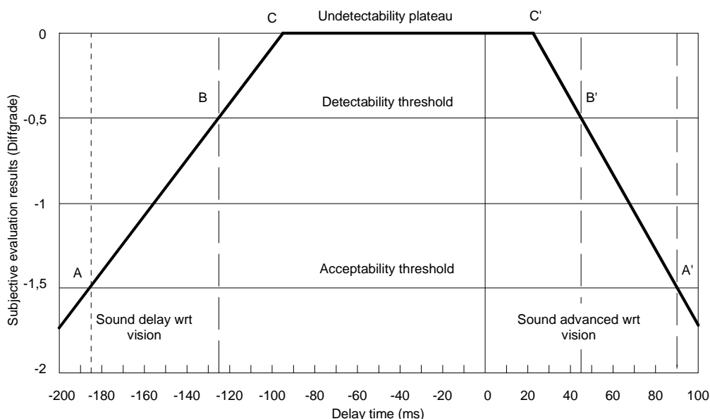
Figure 49: The impact of audio video de-synchronization on perceived quality
