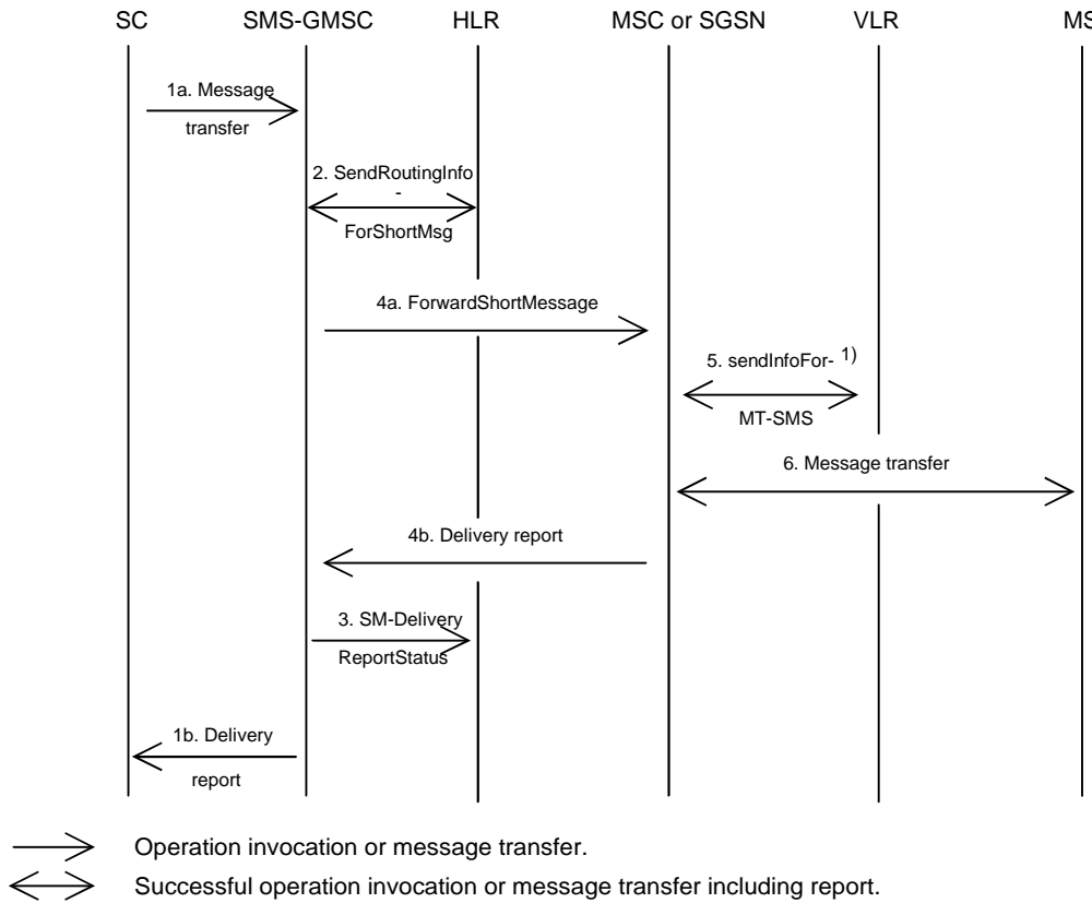
Figure 61: SMS Transaction flow - MT
