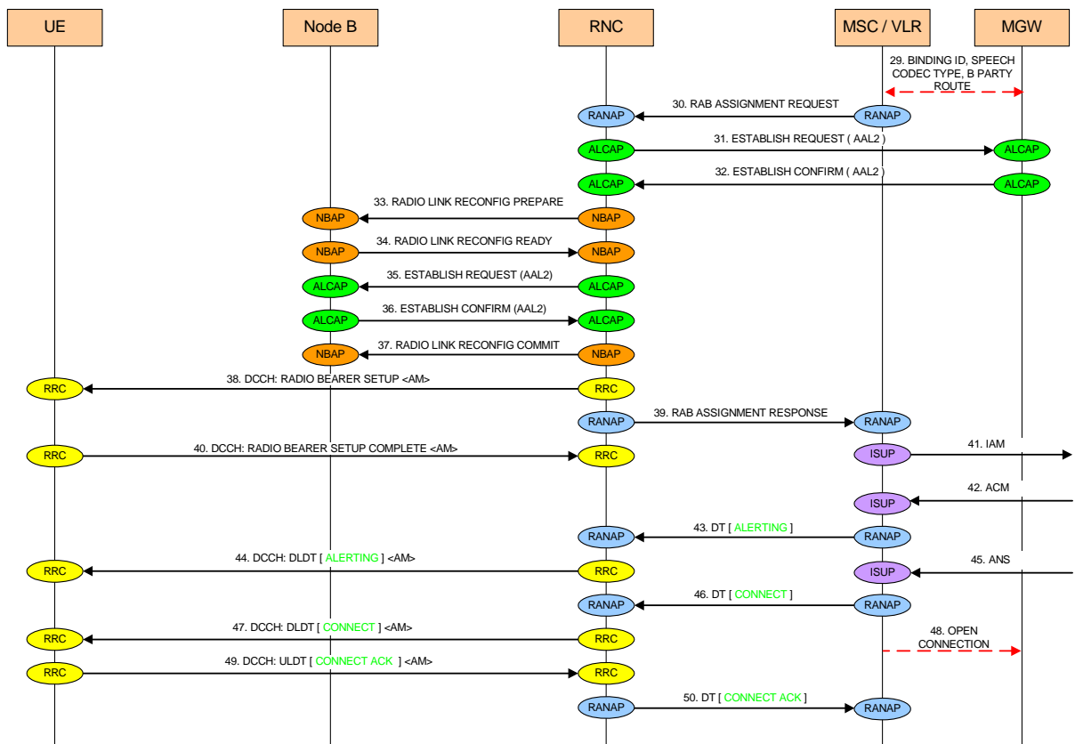
Figure 23: 3G telephony signalling flow chart: mobile originated call establishment procedure
