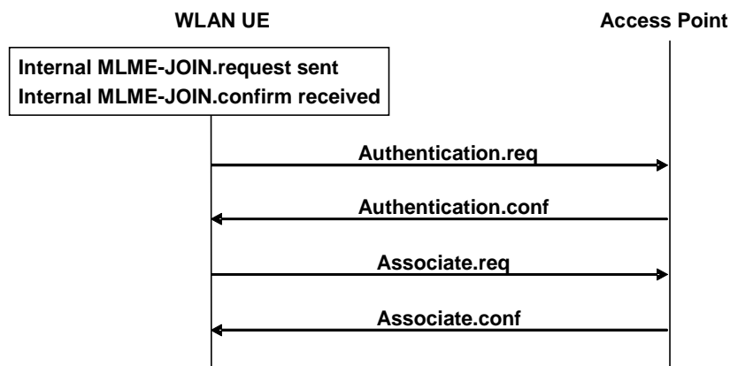
Figure 35: WLAN ASSOCIATION Signal Flow
