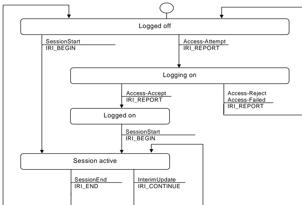
Figure 5: State diagram for an Internet session
