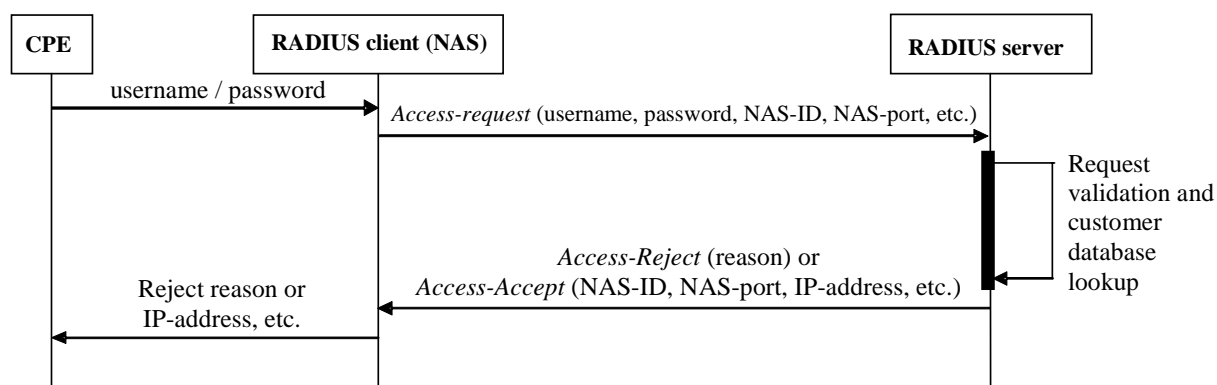
Figure A.3: Basic authentication message exchange
