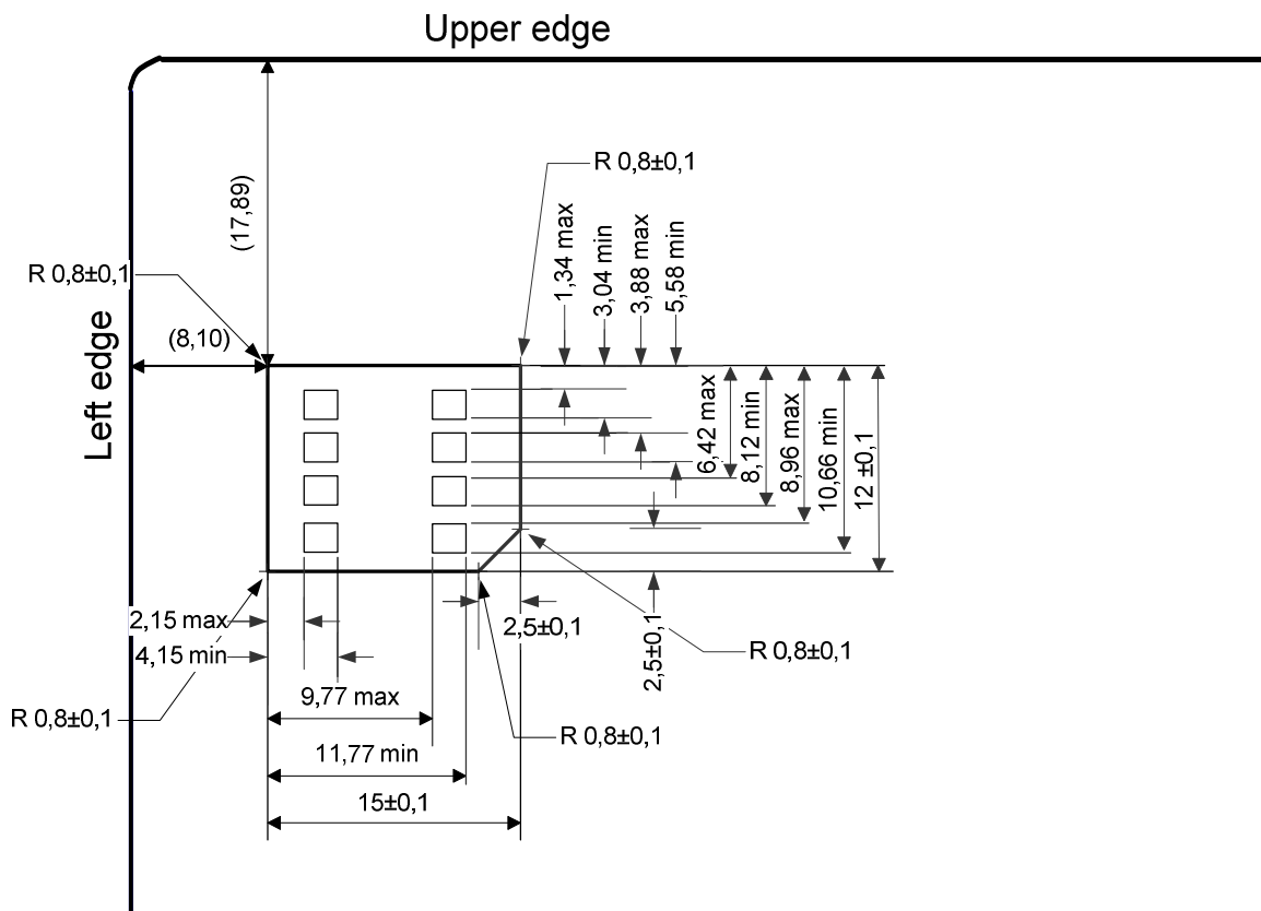
Figure 4.2: Mini-UICC
