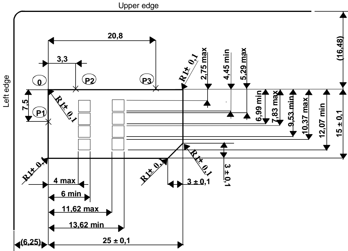
Figure 4.1: Plug-in UICC
