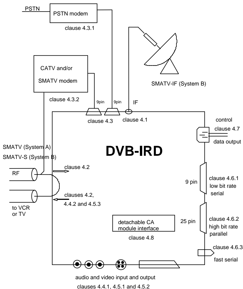
Figure A.1: Generic diagram, showing all optional interfaces
