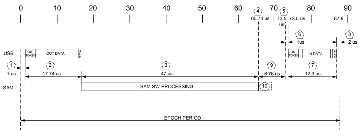
Figure 6.1: ACF timing diagram
