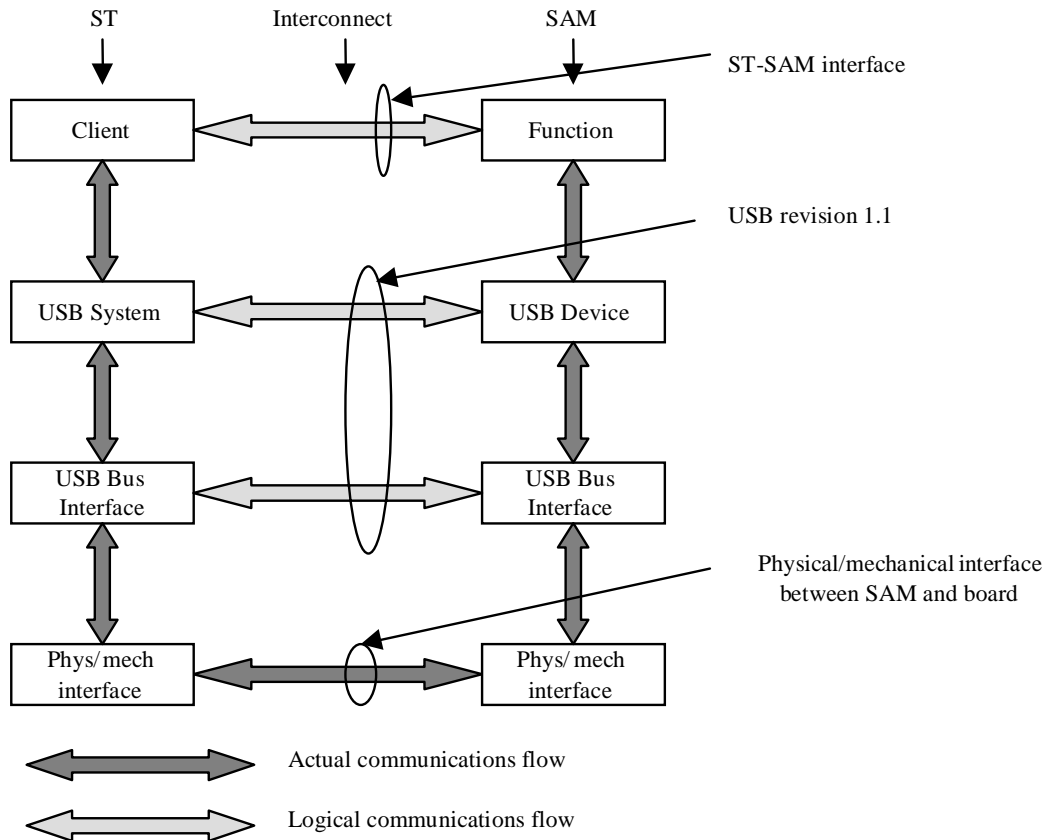
Figure 5.1: Interlayer communications model
