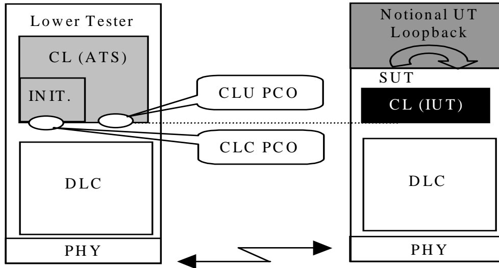
Figure 1: Test architecture for Cell CL – UNI SSCS
