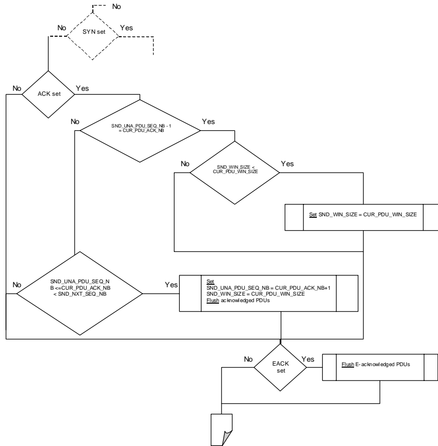
Figure 27: OPEN state PDU arrival event processing 3/4
