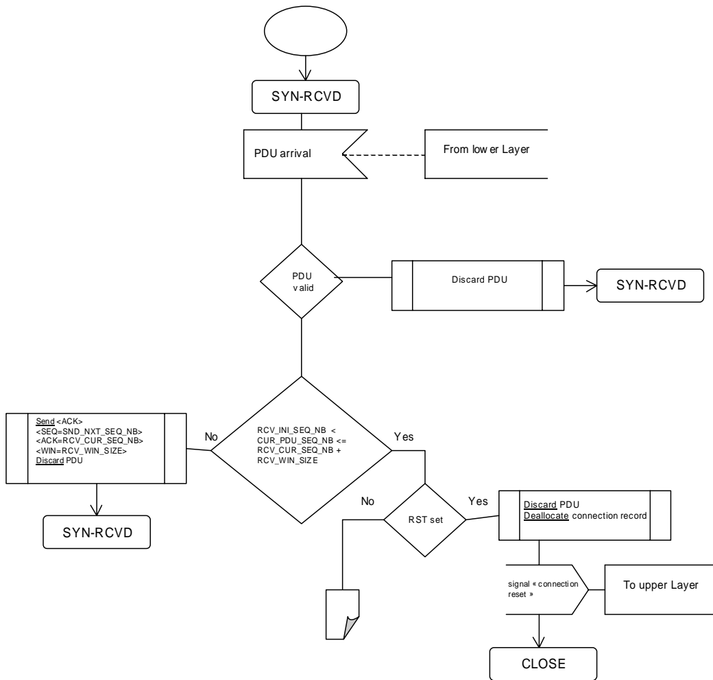
Figure 31: SYN-RCVD state PDU arrival event processing 1/4
