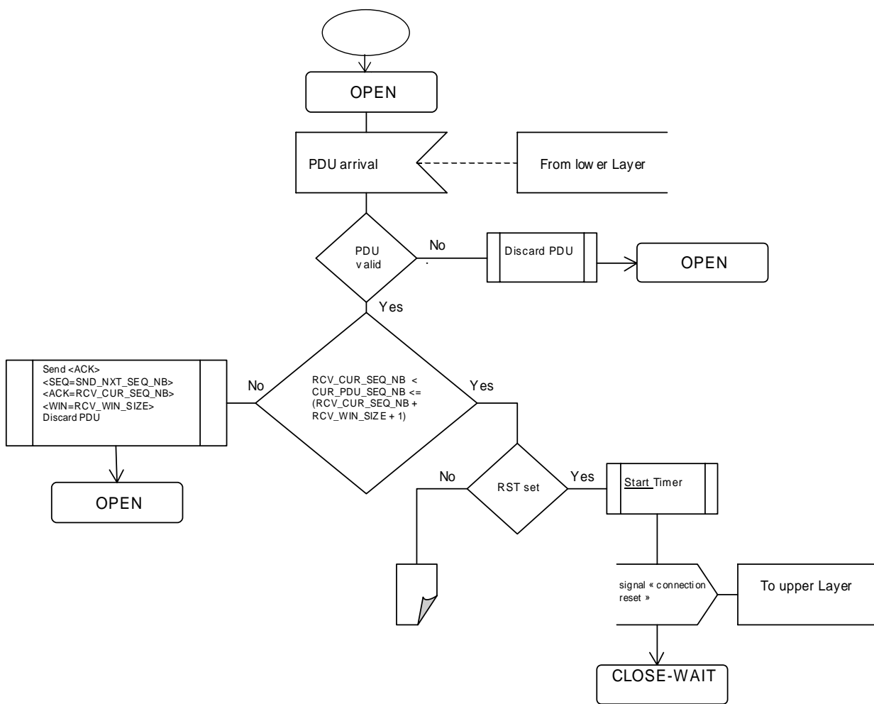
Figure 25: OPEN state PDU arrival event processing 1/4
