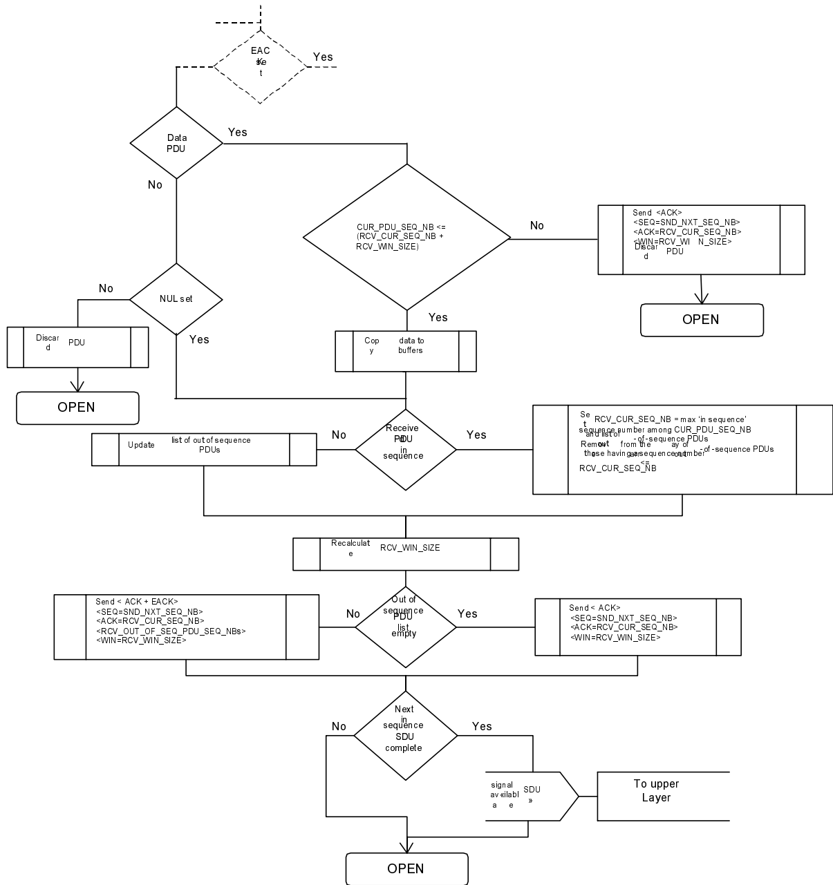
Figure 28: OPEN state PDU arrival event processing 4/4
