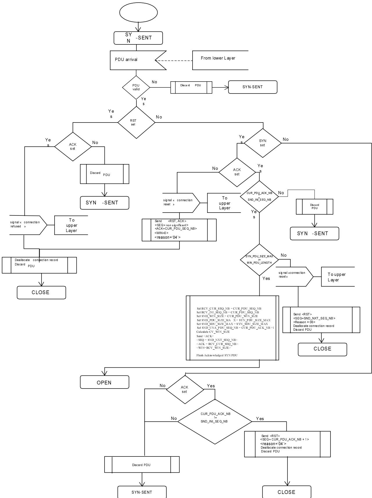
Figure 30: SYN-SENT state PDU arrival event processing
