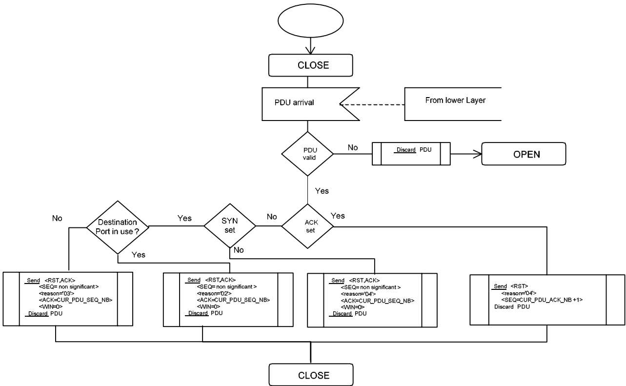
Figure 24: CLOSE state PDU arrival event processing
