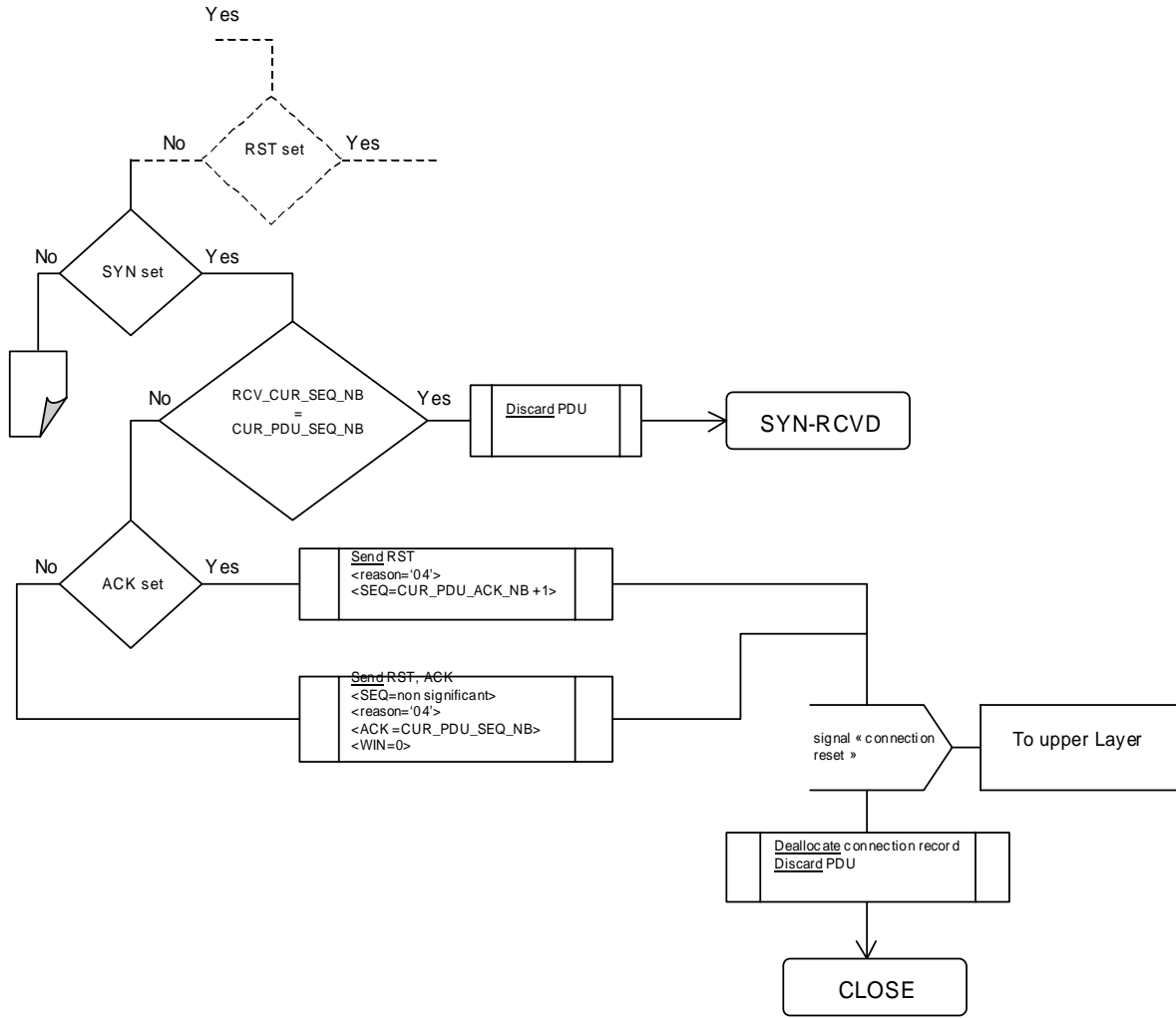
Figure 32: SYN-RCVD state PDU arrival event processing 2/4
