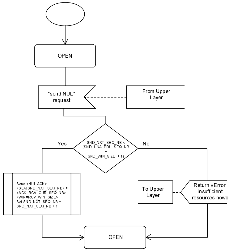
Figure 21a: Send NUL request in OPEN state
