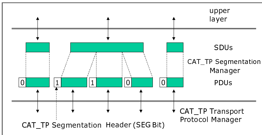
Figure 7: Segmentation description
