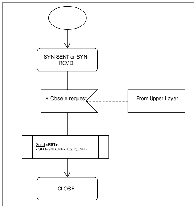
Figure 15: Close request in SYN-SENT or SYN-RCVD state
