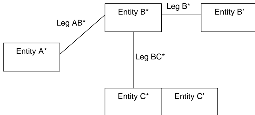
Figure 4: Generalized model for QSIG Single Step Call Transfer
