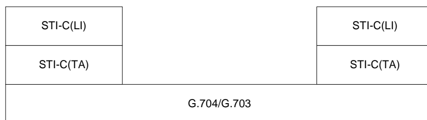
Figure C.2.1: STI-C using the STI-C(TA) over G.704 [6] or G.703 [7]
