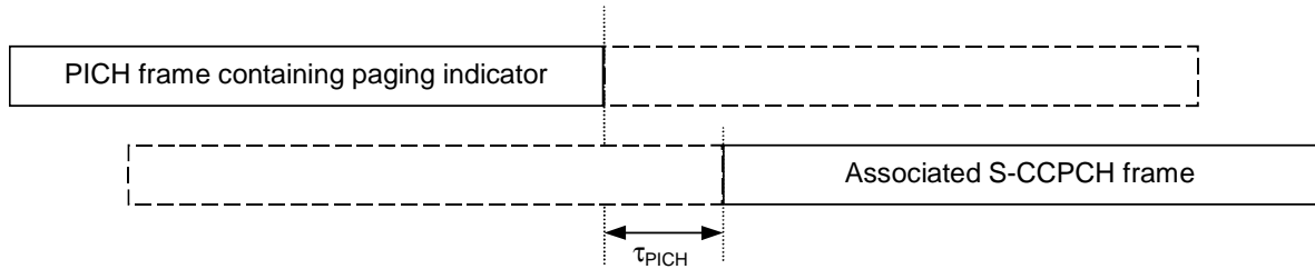
Figure 18: Timing relation between PICH frame and associated S-CCPCH frame
