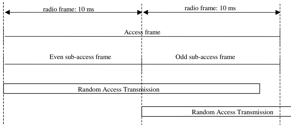
Figure 4a: Structure of the random-access transmission (Optional mode C)
