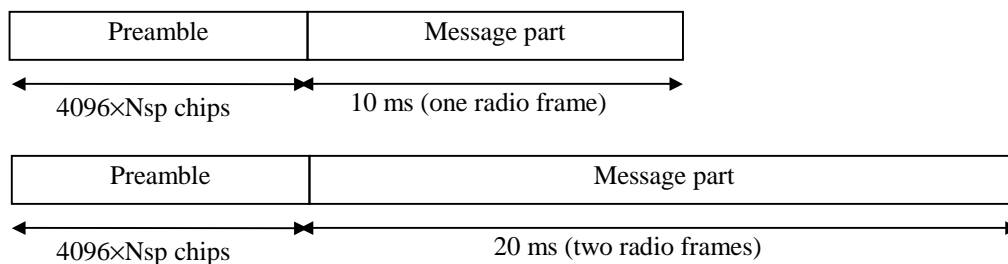
Figure 4b: Structure of the random-access transmission (Optional mode C)
