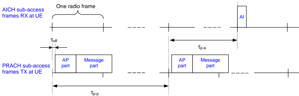
Figure 19a: Timing relation between PRACH and AICH as seen at the UE (Optional mode C)
