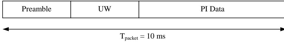
Figure 13a: Packet structure for HPPICH
