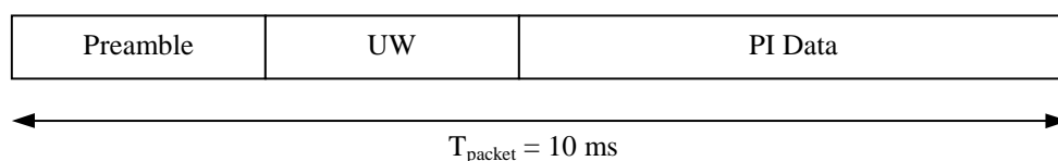
Figure 12: Packet structure for HPPICH
