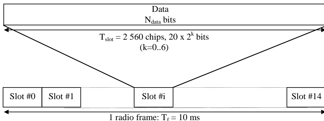
Figure 10: Frame structure for the PDSCH
