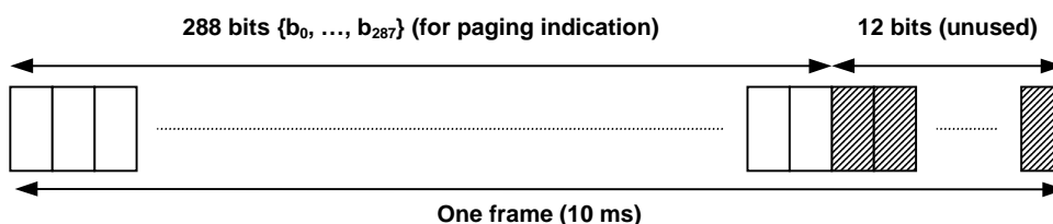
Figure 11: Structure of Page Indicator Channel (PICH)
