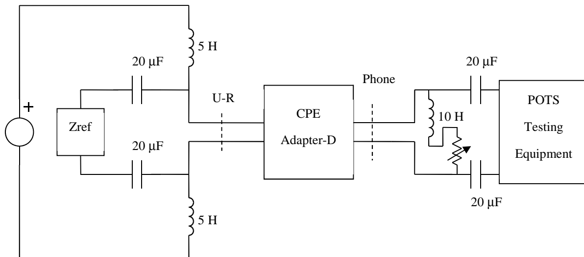
Figure 48: Testing of CPE POTS Adapter-D Characteristics
