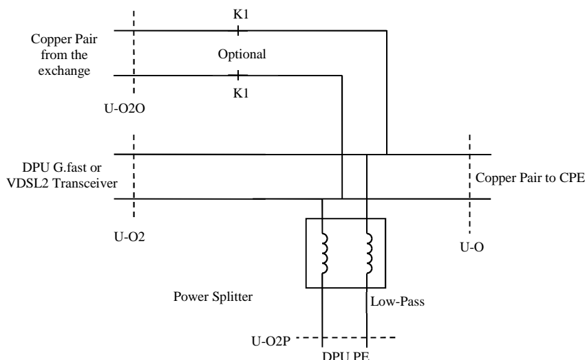
Figure 34: DPU Power Splitter without POTS on the same Pair
