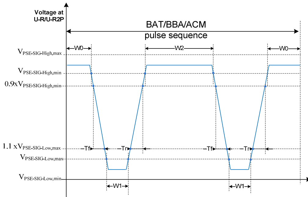
Figure 24: Pulse sequence waveform for BAT, ACM and BBA primitives
