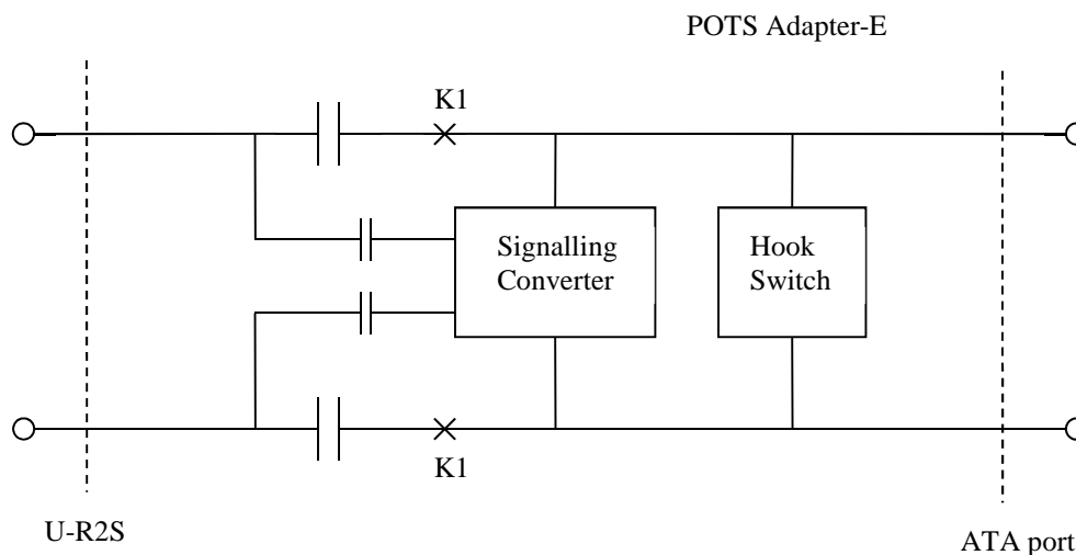
Figure 46: POTS Adapter-E for derived POTS from an ATA
