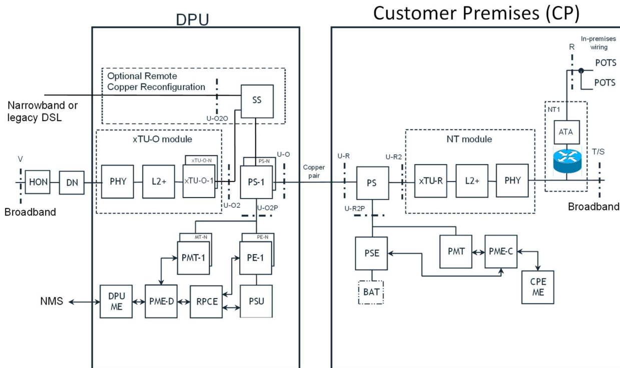
Figure 29: Modified RPFA-DRP Reference Model with derived POTS distributed over In Premises Wiring
