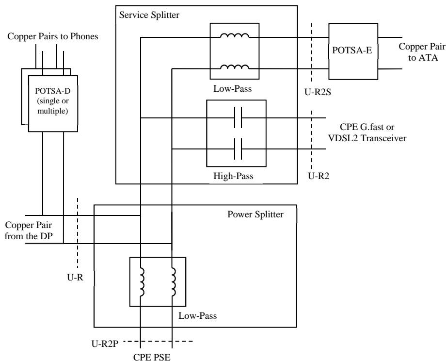
Figure 39: CPE Power Splitter with Derived POTS Sharing the in-premises Wiring
