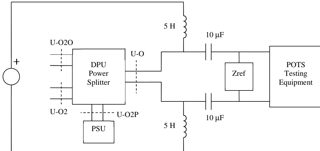
Figure 40: Testing of DPU Power Splitter POTS Characteristics
