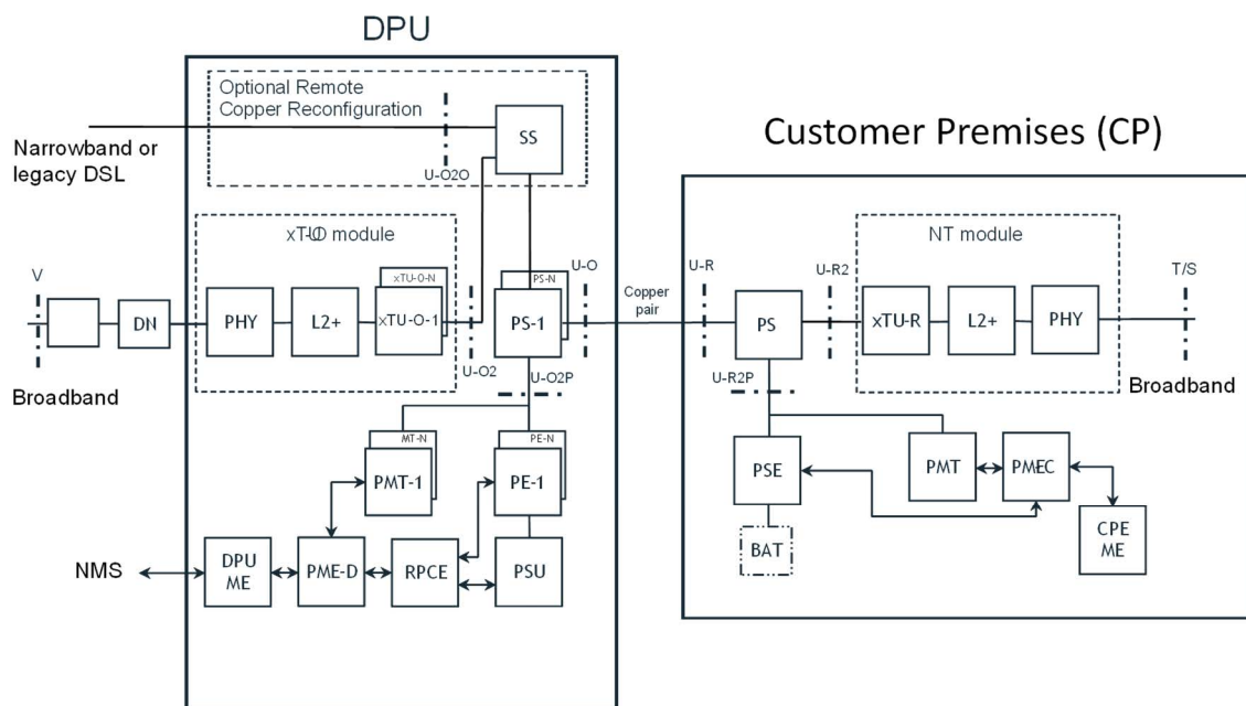
Figure 27: Modified RPFA-NOP Reference Model
