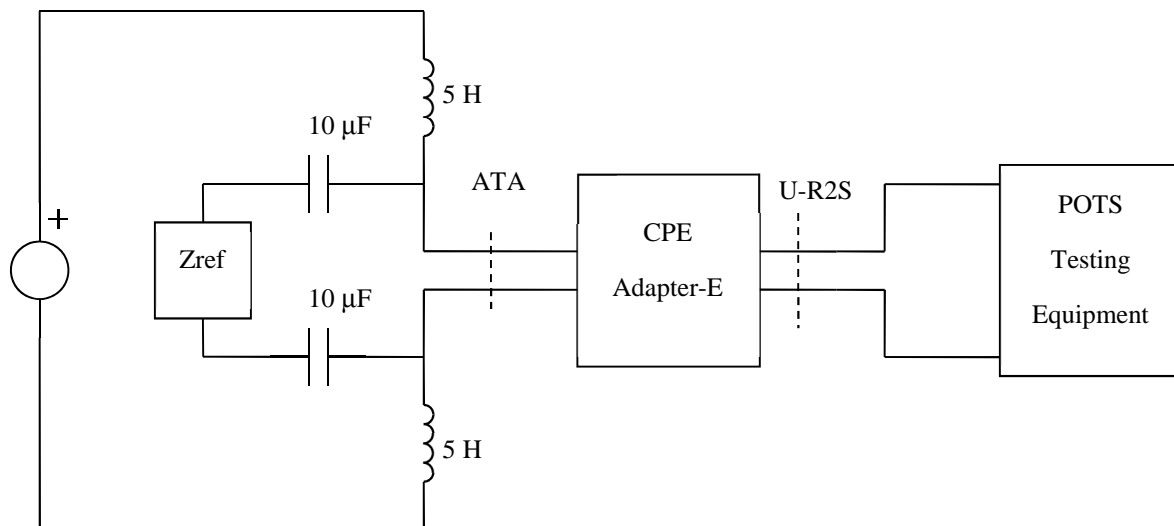
Figure 50: Testing of CPE POTS Adapter-E Characteristics
