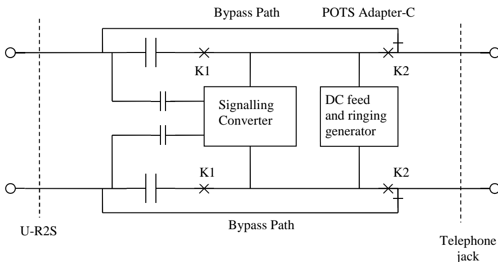
Figure 43: POTS Adapter-C for POTS from the exchange
