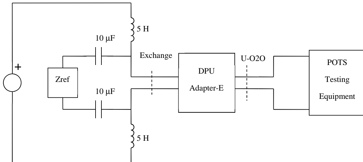
Figure 49: Testing of DPU POTS Adapter-E Characteristics
