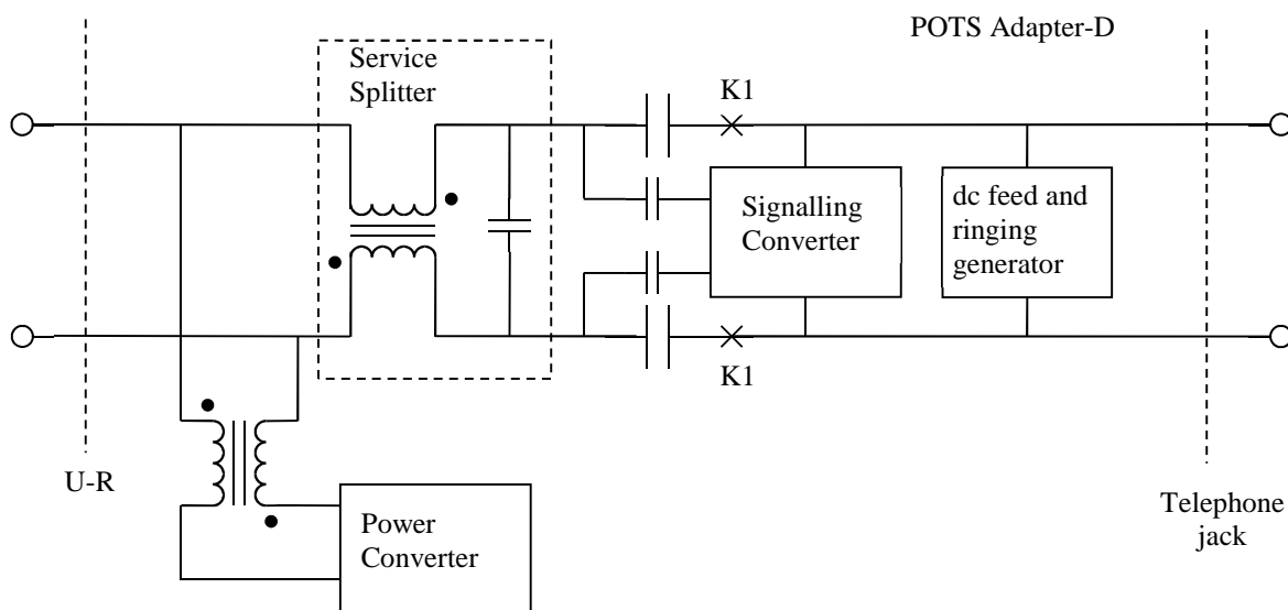
Figure 45: POTS Adapter-D for derived POTS from an ATA
