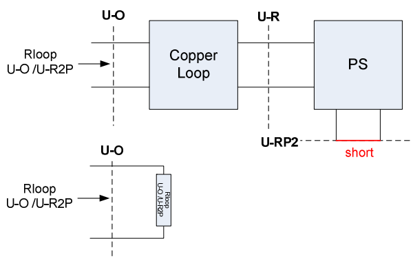
Figure 32: Loop resistance U-R2P to U-O interface
