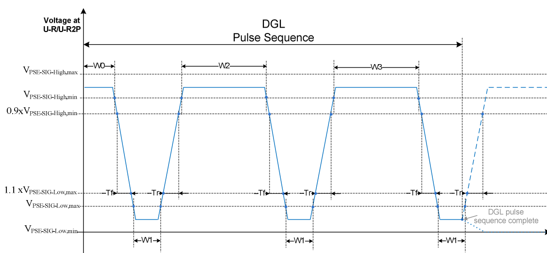
Figure 22: Pulse sequence waveform for DGL primitive
