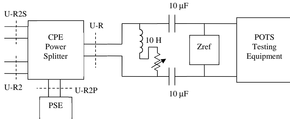
Figure 41: Testing of CPE Power Splitter POTS Characteristics
