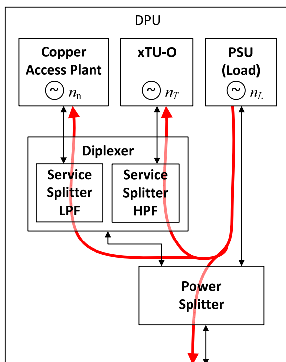
Figure 26: Example of noise coupling paths in a zero touch Integration
