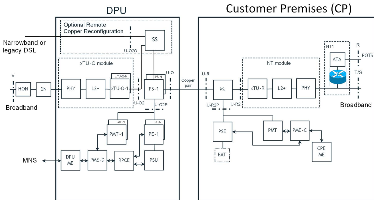
Figure 28: Modified RPFA-DRP Reference Model with derived POTS and a single POTS port
