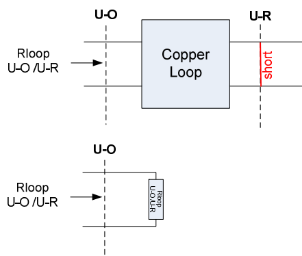
Figure 33: Loop resistance U-R to U-O interface
