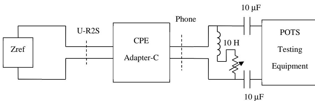
Figure 47: Testing of CPE POTS Adapter-C Characteristics
