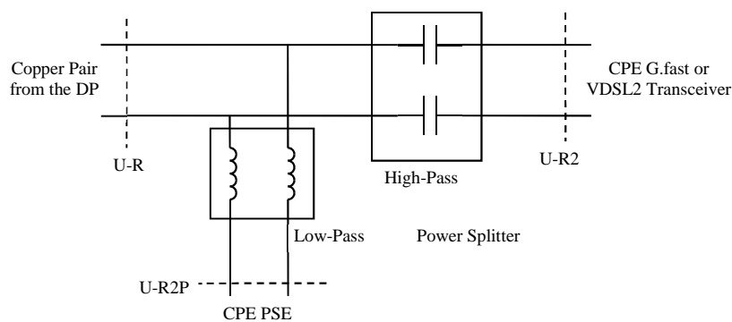
Figure 37: CPE Power Splitter without POTS on the same Pair
