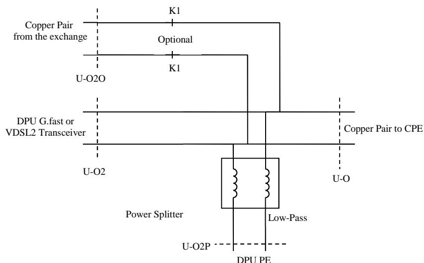
Figure 36: DPU Power Splitter with Derived POTS
