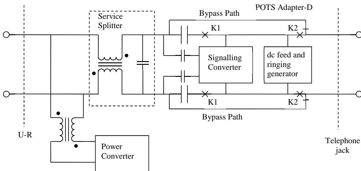
Figure 44: POTS Adapter-D for POTS from the exchange
