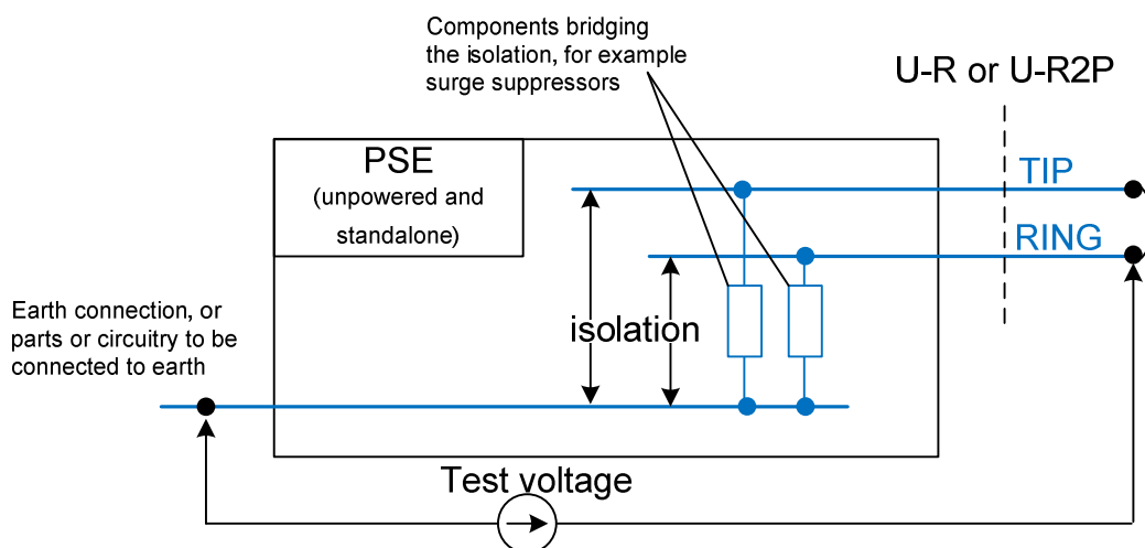
Figure 31: DC resistance between Earth and U-R/UR-2P
