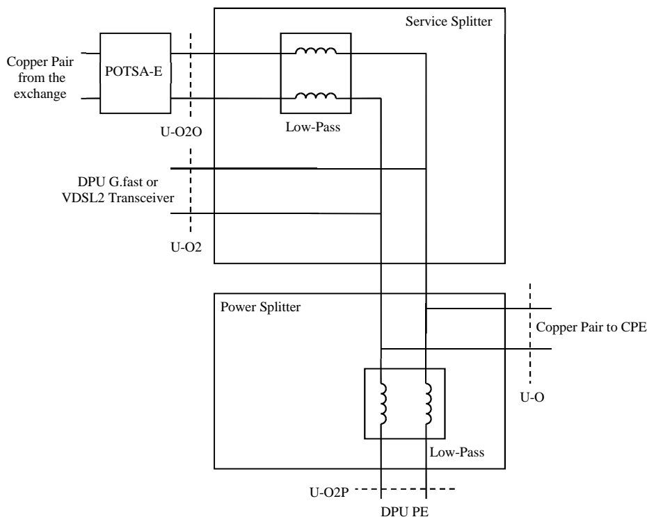
Figure 35: DPU Power Splitter with POTS from the Exchange
