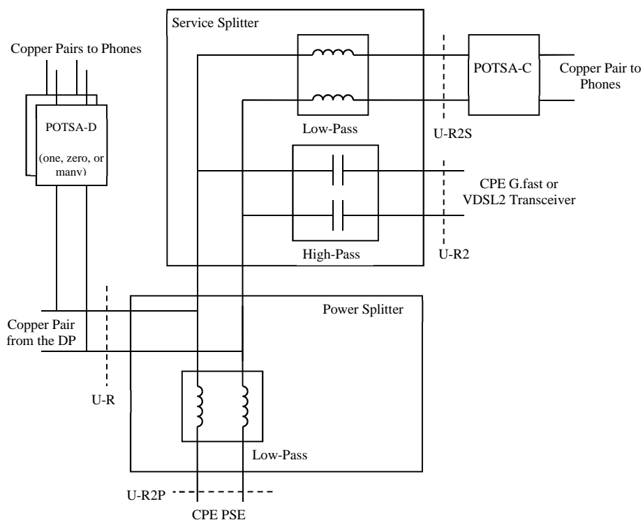
Figure 38: CPE Power Splitter with POTS from the Exchange
