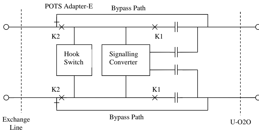
Figure 42: DPU POTS Adapter-E for POTS from the exchange
