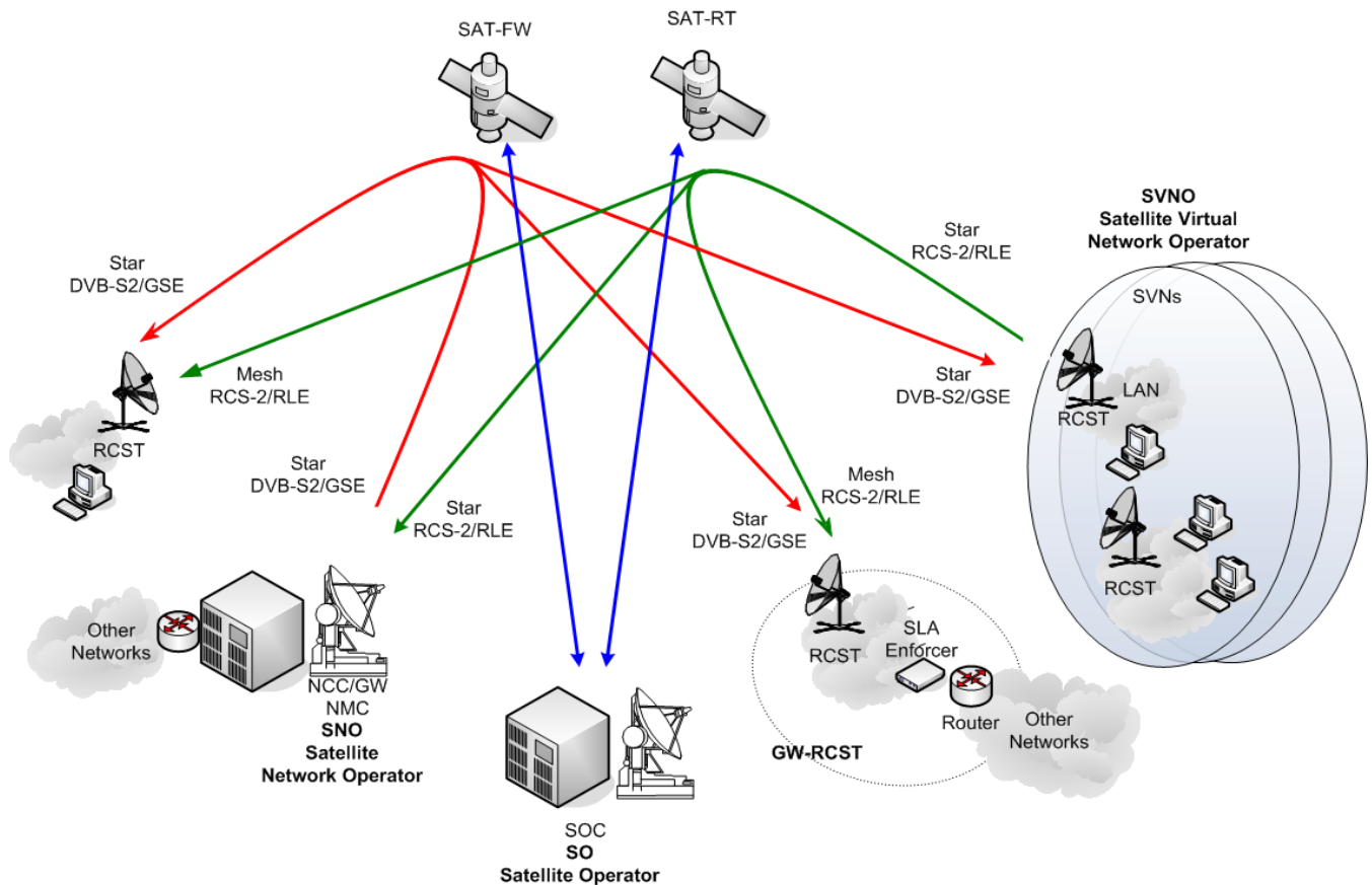
Figure 1: Main roles in a DVB-RCS2 transparent satellite interactive network
