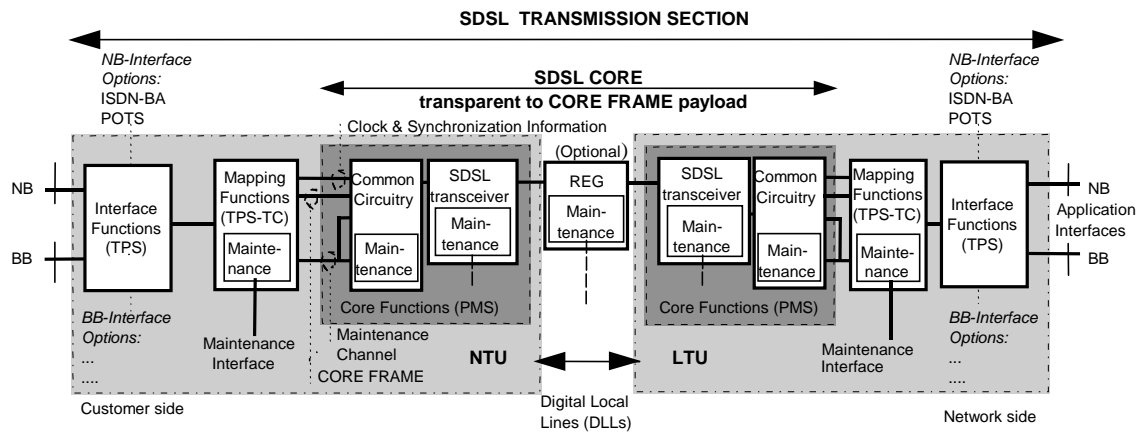
Figure 4-4: Protocol reference model
