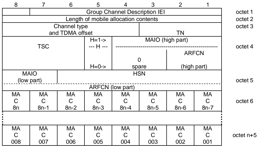
Figure 10.5.41/GSM 04.18: Group Channel Description information element
