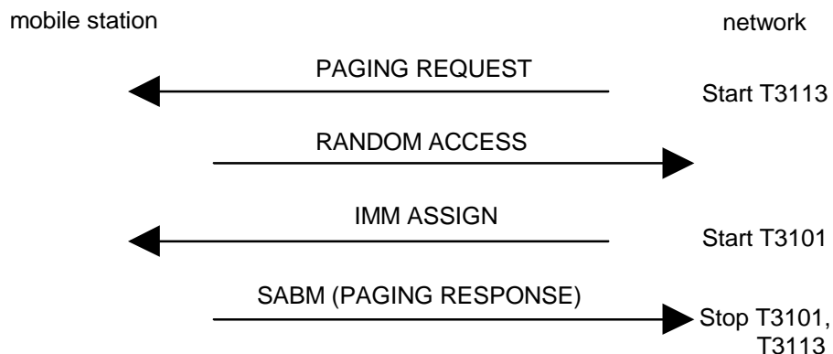
Figure 3.2/GSM 04.18: Paging sequence
