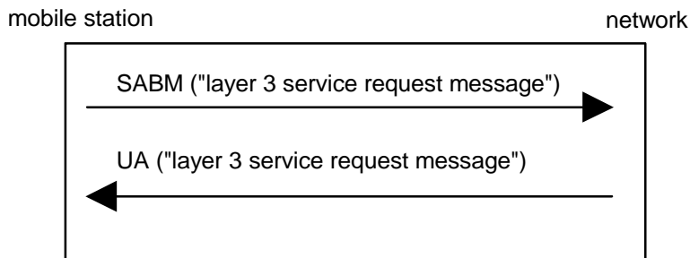
Figure 3.1/GSM 04.18: Service request and contention resolution
