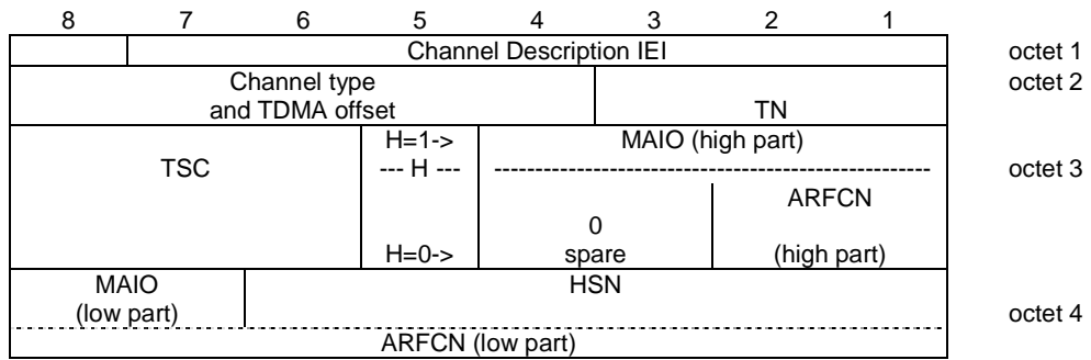
Figure 10.5.26/GSM 04.18: Channel Description 2 information element
