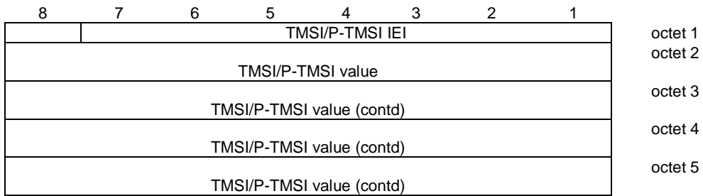
Figure 10.5.70/GSM 04.18: TMSI/P-TMSI information element
