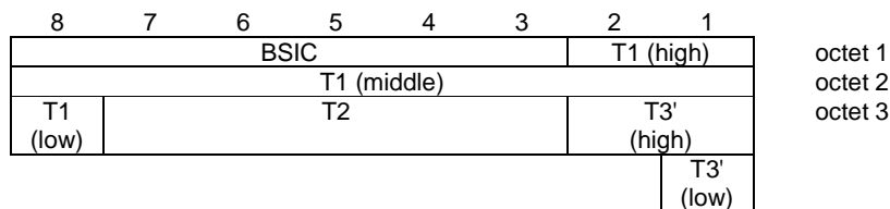
Figure 9.3a/GSM 04.18: Frame synchronization information element
