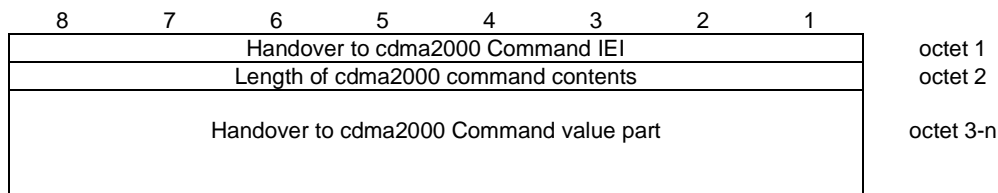
Figure 10.5.2.52/GSM 04.18: Handover to cdma2000 Command information element
