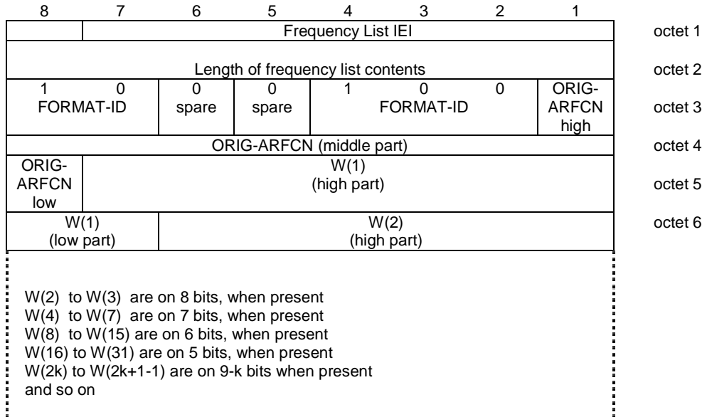
Figure 10.5.37/GSM 04.18: Frequency List information element (Range 512 format)
