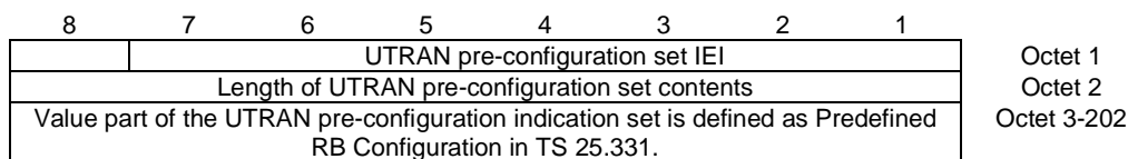
Figure 10.5.27/GSM 04.18: UTRAN pre-configuration set information element
