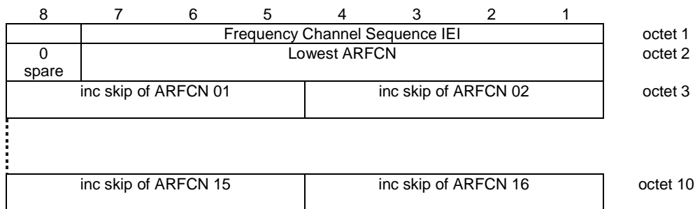
Figure 10.5.34/GSM 04.18: Frequency Channel Sequence information element
