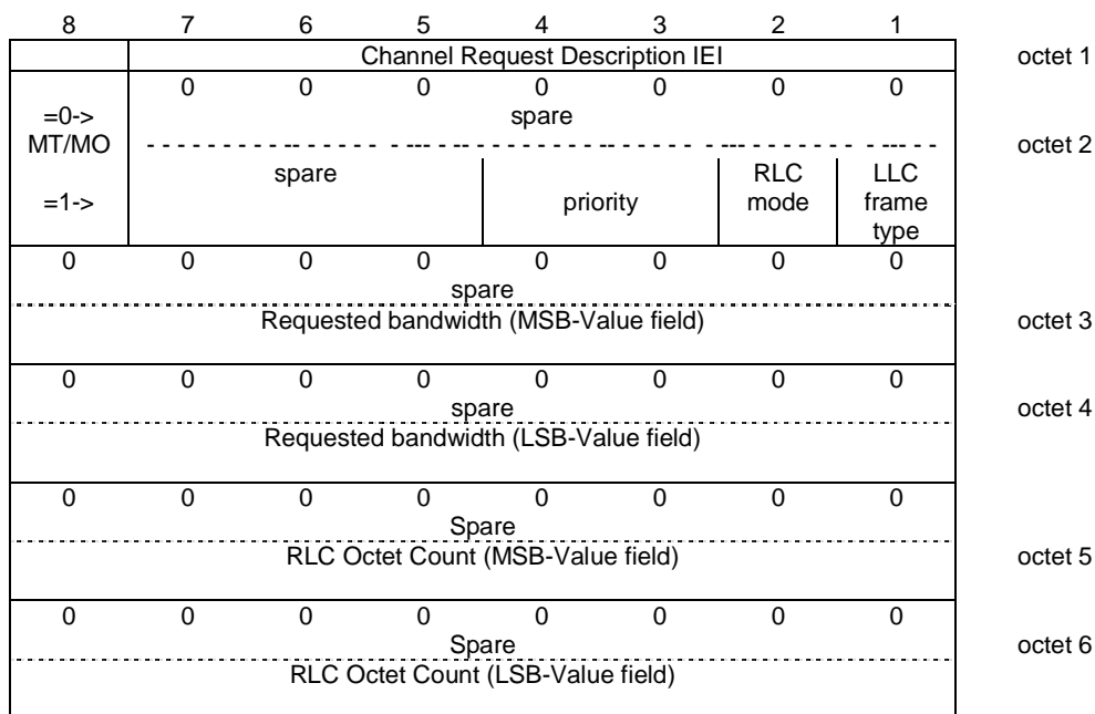
Figure 10.5.30/GSM 04.18: Channel Request Description information element
