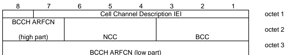
Figure 10.5.20/GSM 04.18: Cell Description information element
