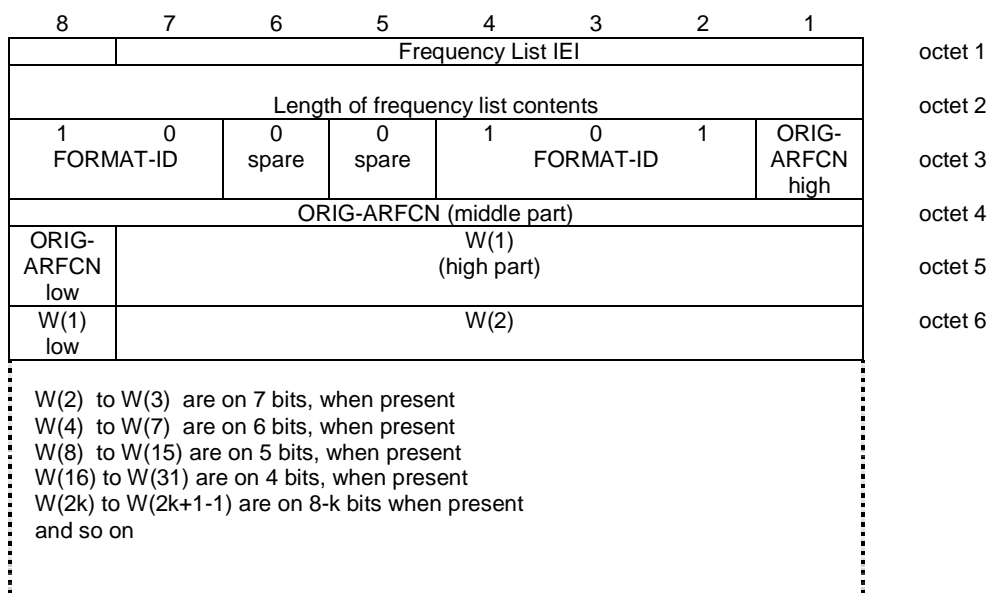
Figure 10.5.38/GSM 04.18: Frequency List information element (Range 256 format)
