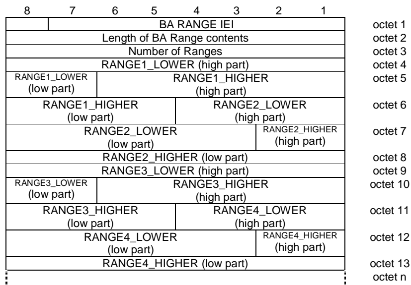
Figure 10.5.12/GSM 04.18: BA RANGE information element
