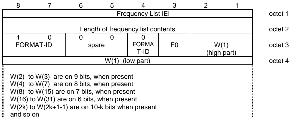
Figure 10.5.36/GSM 04.18: Frequency List information element (Range 1024 format)
