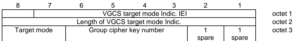
Figure 10.5.71/GSM 04.18: VGCS target mode Indication information element
