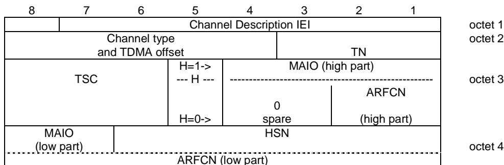
Figure 10.5.25/GSM 04.18: Channel Description information element
