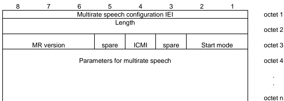
Figure 10.5.2.47/GSM 04.18: MultiRate configuration information element
