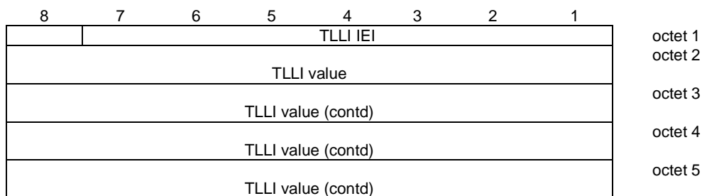
Figure 10.5.69/GSM 04.18: TLLI information element
