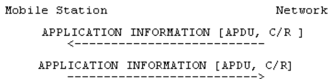
Figure 3.4/GSM 04.18: Application Information Transfer without segmentation
