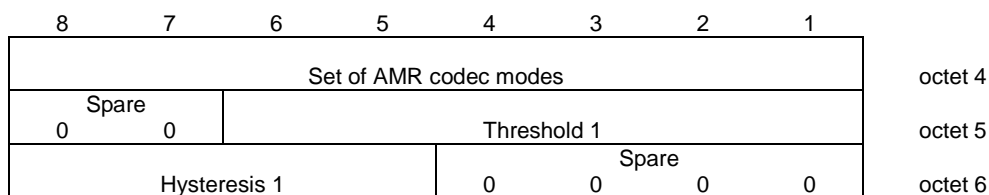
Figure 10.5.2.47b/GSM 04: Parameters for multirate speech field for the MR version 1 when a set with two codec modes is chosen
