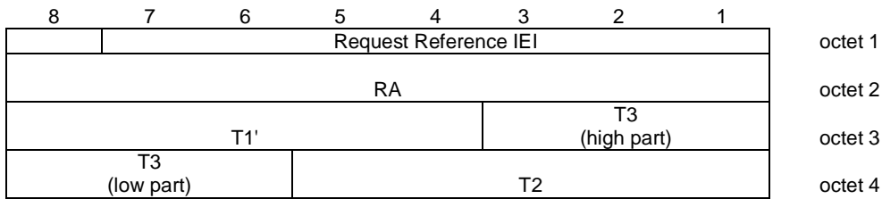
Figure 10.5.61/GSM 04.18: Request Reference information element
