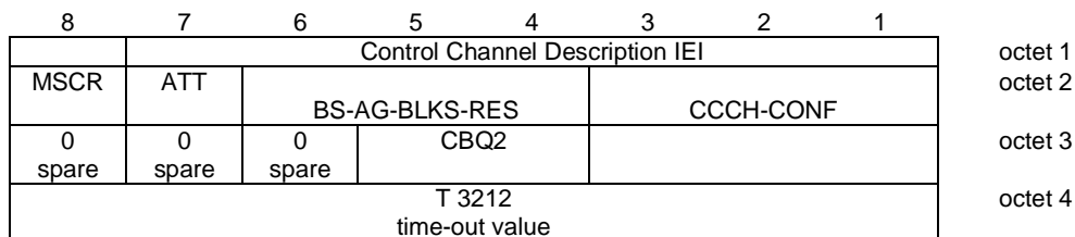
Figure 10.5.33/GSM 04.18: Control Channel Description information element
