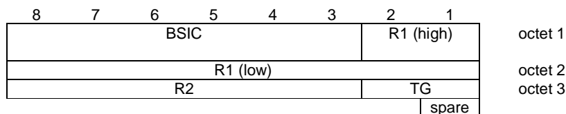
Figure 9.3b/GSM 04.18: COMPACT Frame synchronization information element
