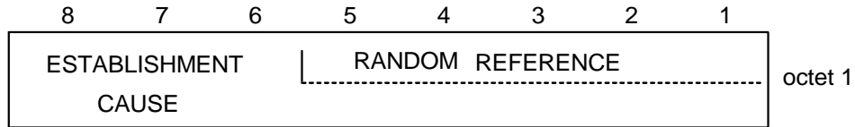
Figure 9.4/GSM 04.18: UPLINK ACCESS message content
