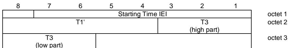
Figure 10.5.65/GSM 04.18: Starting Time information element
