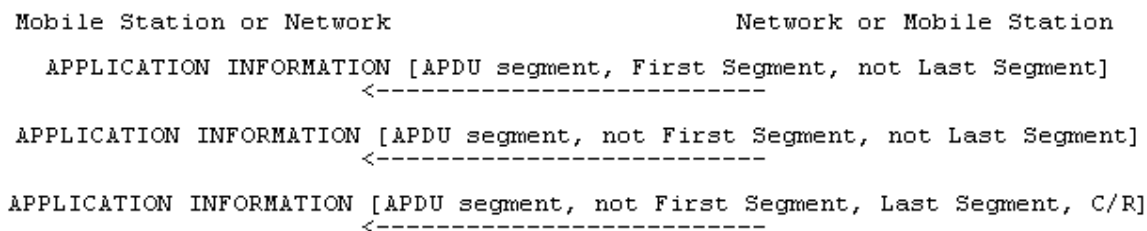
Figure 3.5/GSM 04.18: Application Information Transfer with segmentation
