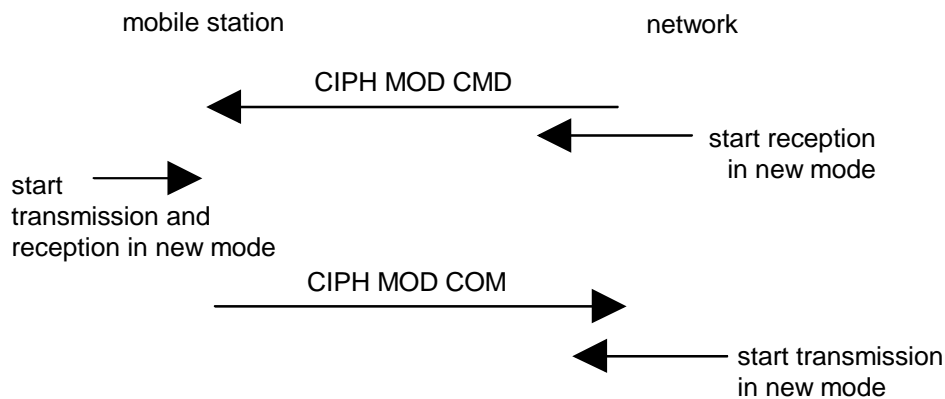
Figure 3.3/GSM 04.18: Cipherng mode setting sequence
