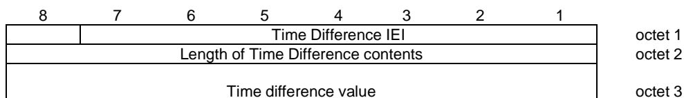
Figure 10.5.68/GSM 04.18: Time Difference information element
