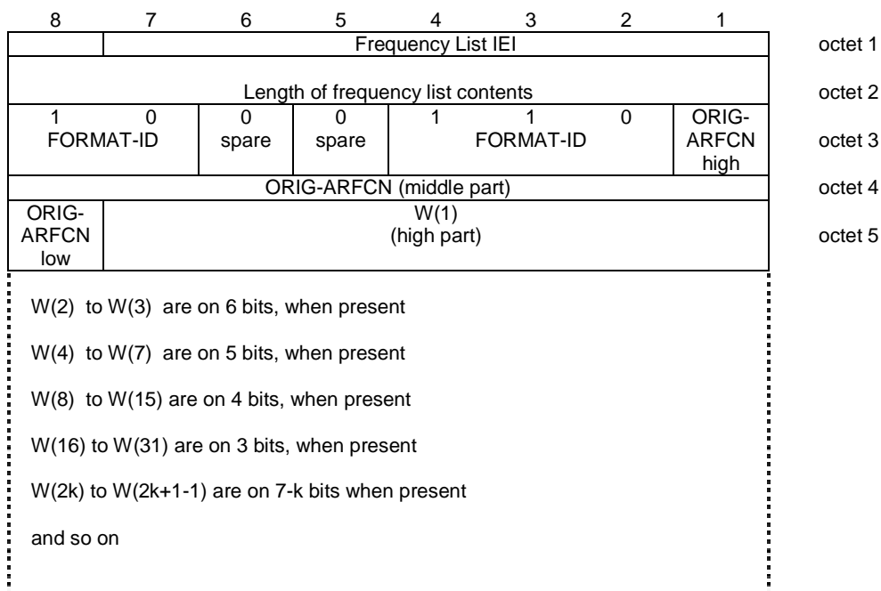
Figure 10.5.39/GSM 04.18: Frequency List information element (Range 128 format)
