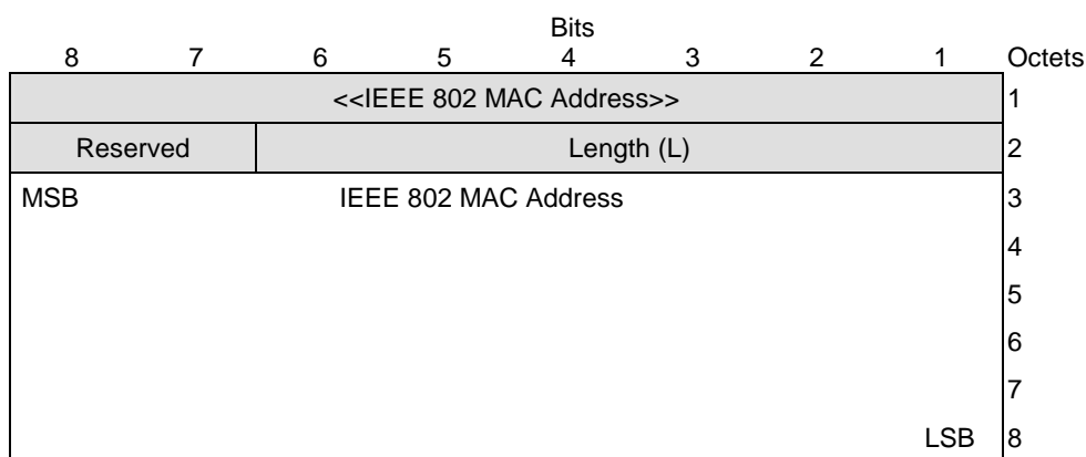
Figure 6.2: IEEE 802 MAC Address information element
