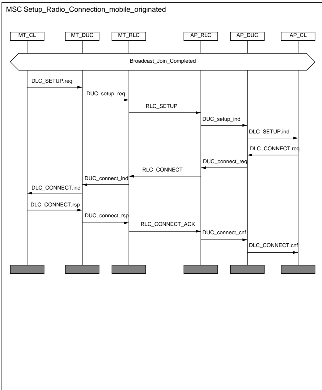
Figure B.4: MT originated DUC setup procedure
