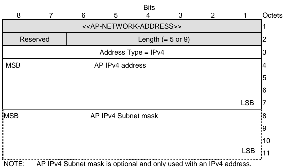
Figure 6.4: AP Network Address information element (for IPv4 address + IPv4 Subnet mask)
