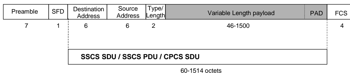
Figure 5.1: IEEE 802.3 frame
