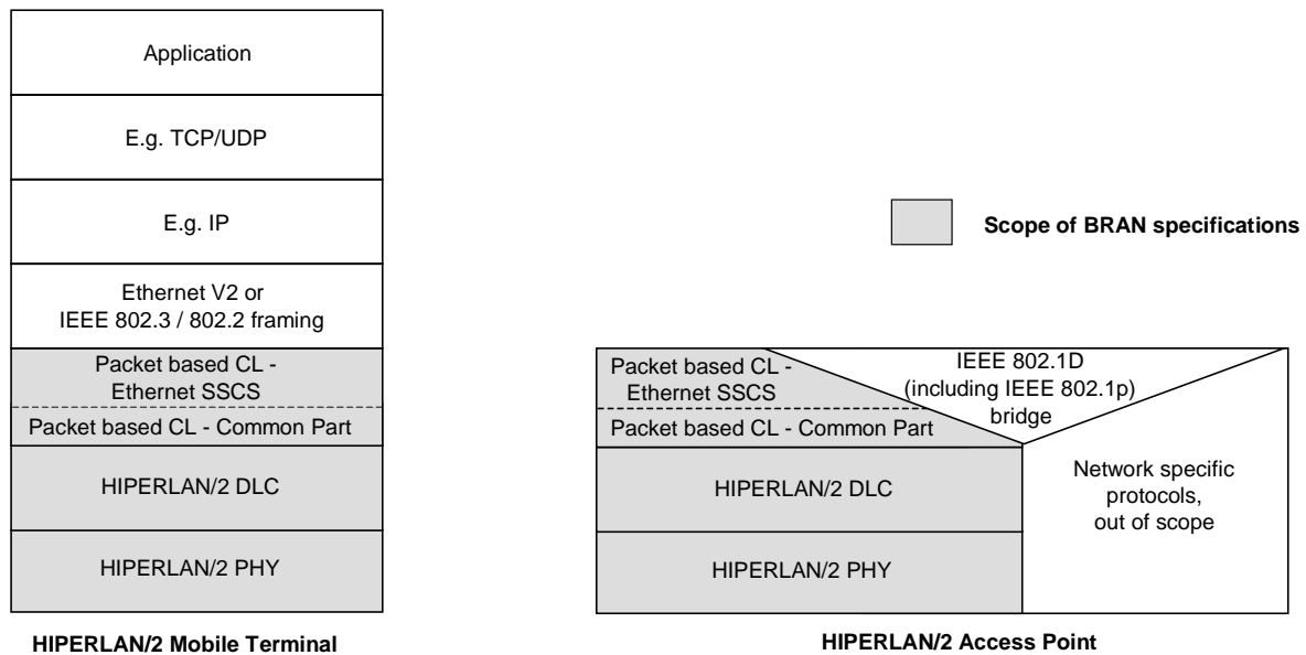
Figure 4.2: Ethernet SACS architecture applied to HIPERLAN/2
