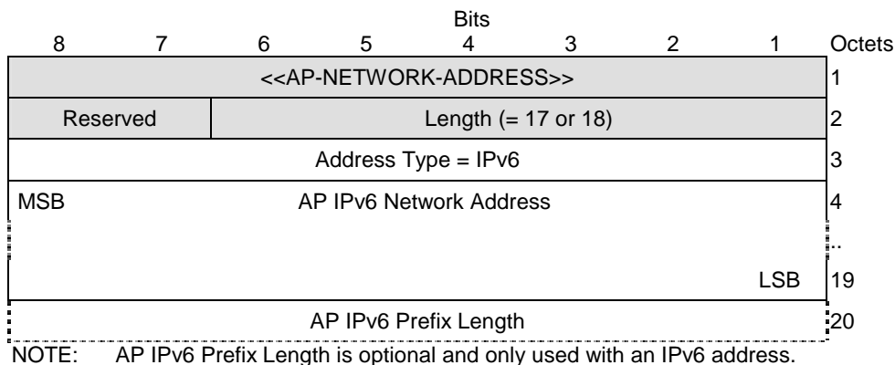
Figure 6.5: AP Network Address information element (for IPv6 address + IPv6 Prefix Length)
