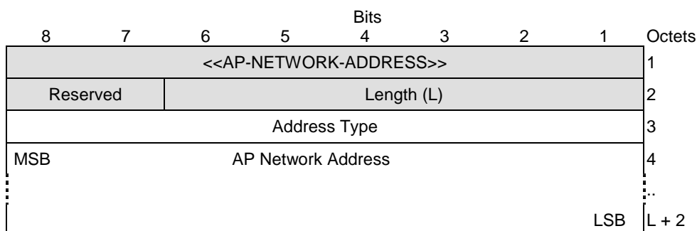
Figure 6.3: AP Network Address information element
