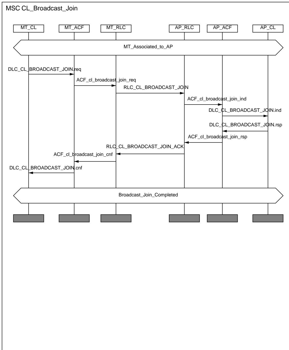
Figure B.3: CL Broadcast Join procedure
