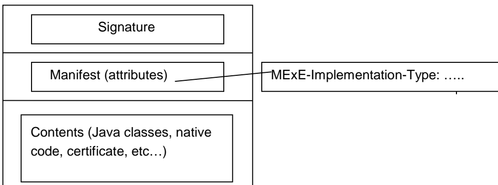
Figure 6: signed packages
