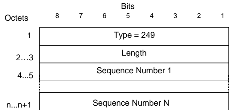
Figure 17: Sequence Numbers of Released Packets information element
