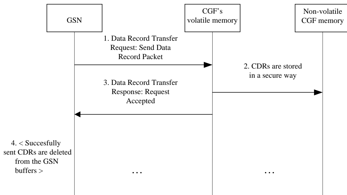
Figure 20: A normal CDR transfer process between a GSN and CGF
