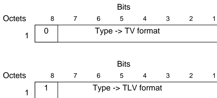
Figure 12: Type field for TV and TLV format
