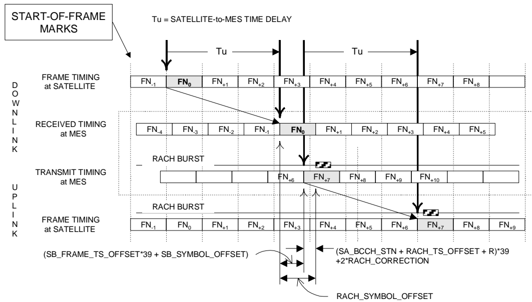
Figure 5.2: RACH burst timing
