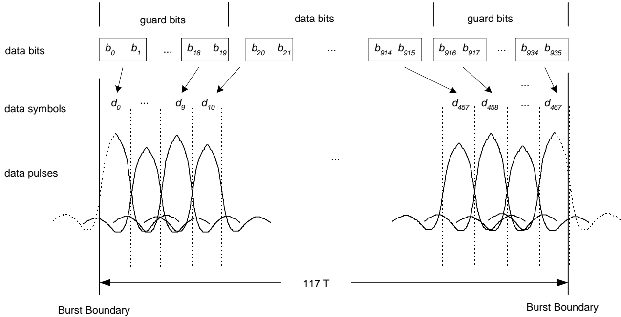
Figure 4.1: Relationship of data bits, data symbols, burst timing, and symbol timing for PNB(4,3)
