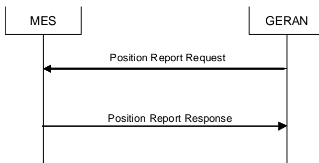
Figure 7.13.2.1: Position Reporting
