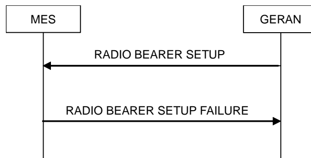
Figure 7.14.1.2: Radio Bearer Establishment, MES reverts to old configuration
