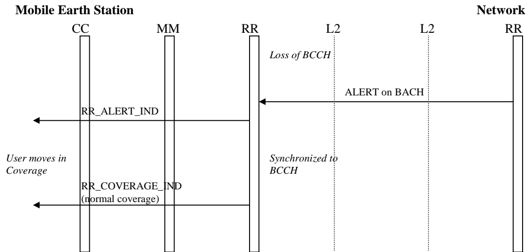
Figure A.9: Alerting. Successful case (see GMR-1 03.298)
