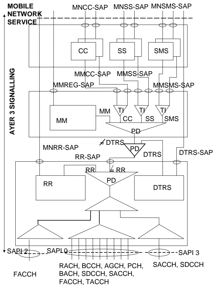
Figure 5.1: Protocol architecture of signalling layer 3 - mobile earth station side
