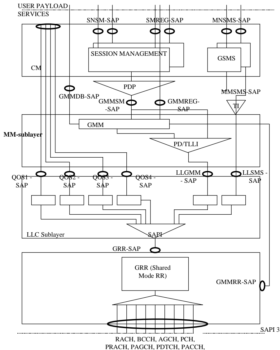
Figure 5.2: Protocol Architecture supporting GMPRS class C MESSs, MES - side
