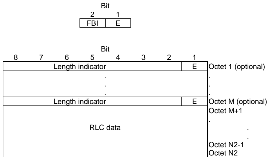
Figure 10: EGPRS downlink RLC data block
