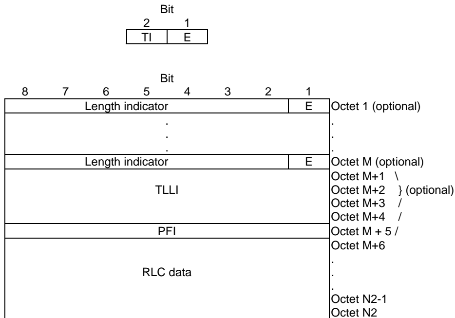
Figure 11: Uplink EGPRS RLC data block
