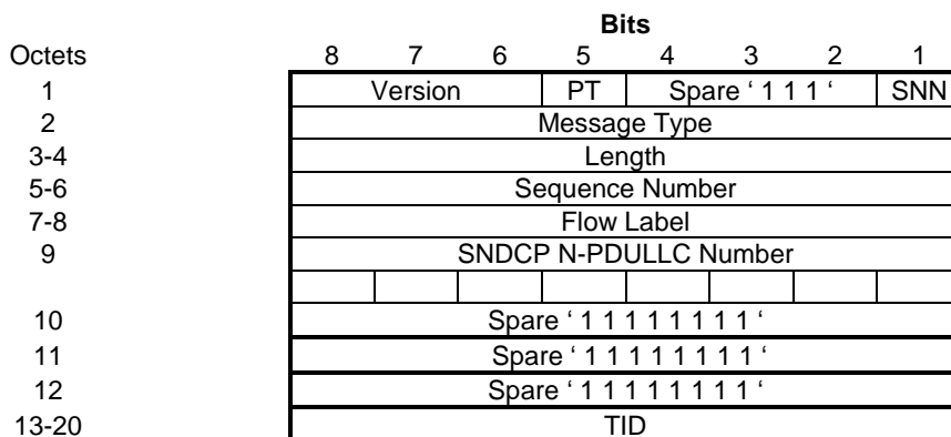
Figure 2: Outline of GTP header
