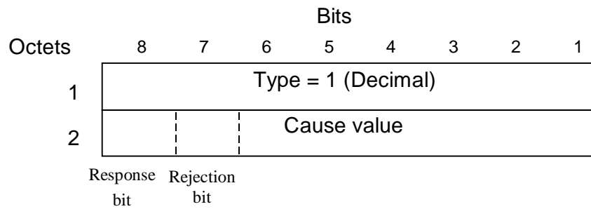
Figure 8: Cause information element
