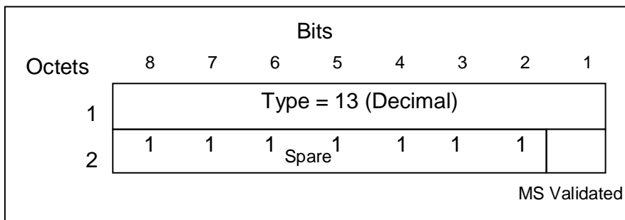
Figure 18: MS Validated information element
