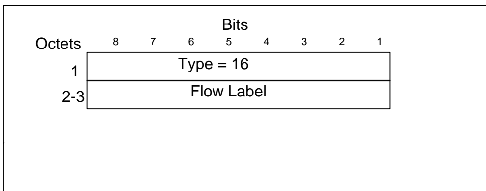
Figure 21: Flow Label Data information element
