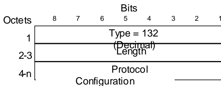
Figure 32: Protocol Configuration Options information element
