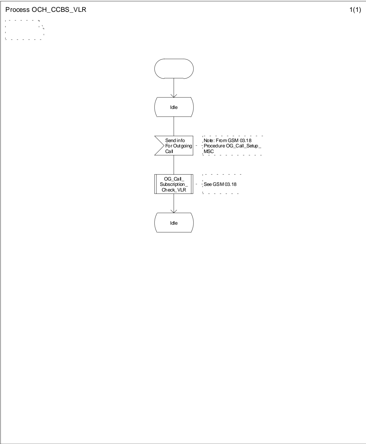
Figure 11.1.1.3: Process OCH_CCBS_VLR
