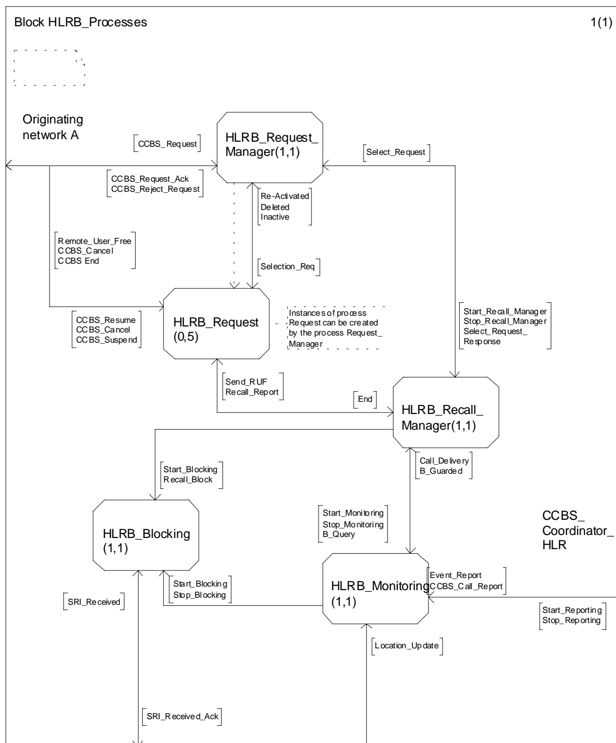
Figure 11.2.2.1: HLRB_Processes
