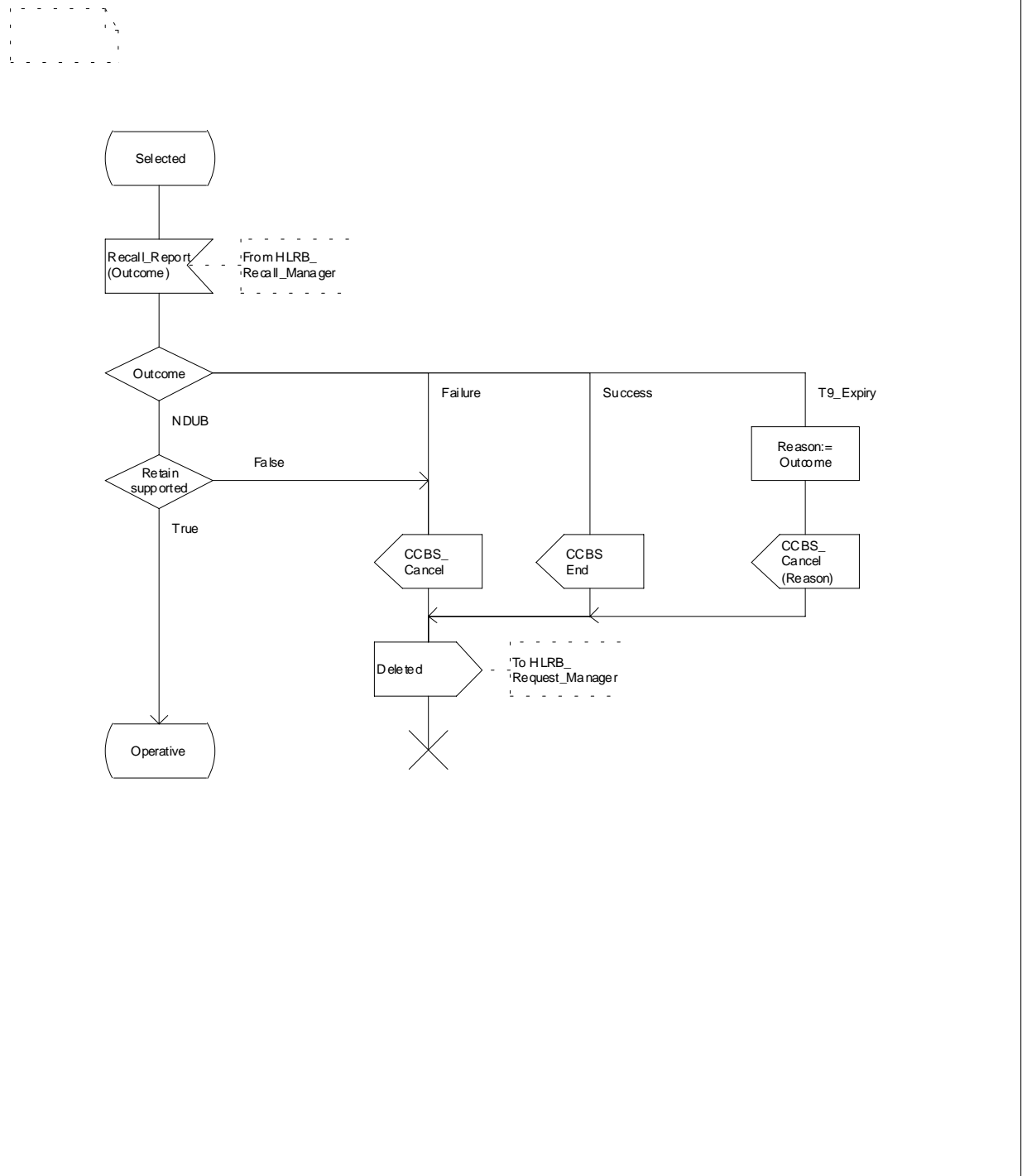
Figure 11.2.2.3: Process HLRB_REQUEST (sheet 4 of 6)
