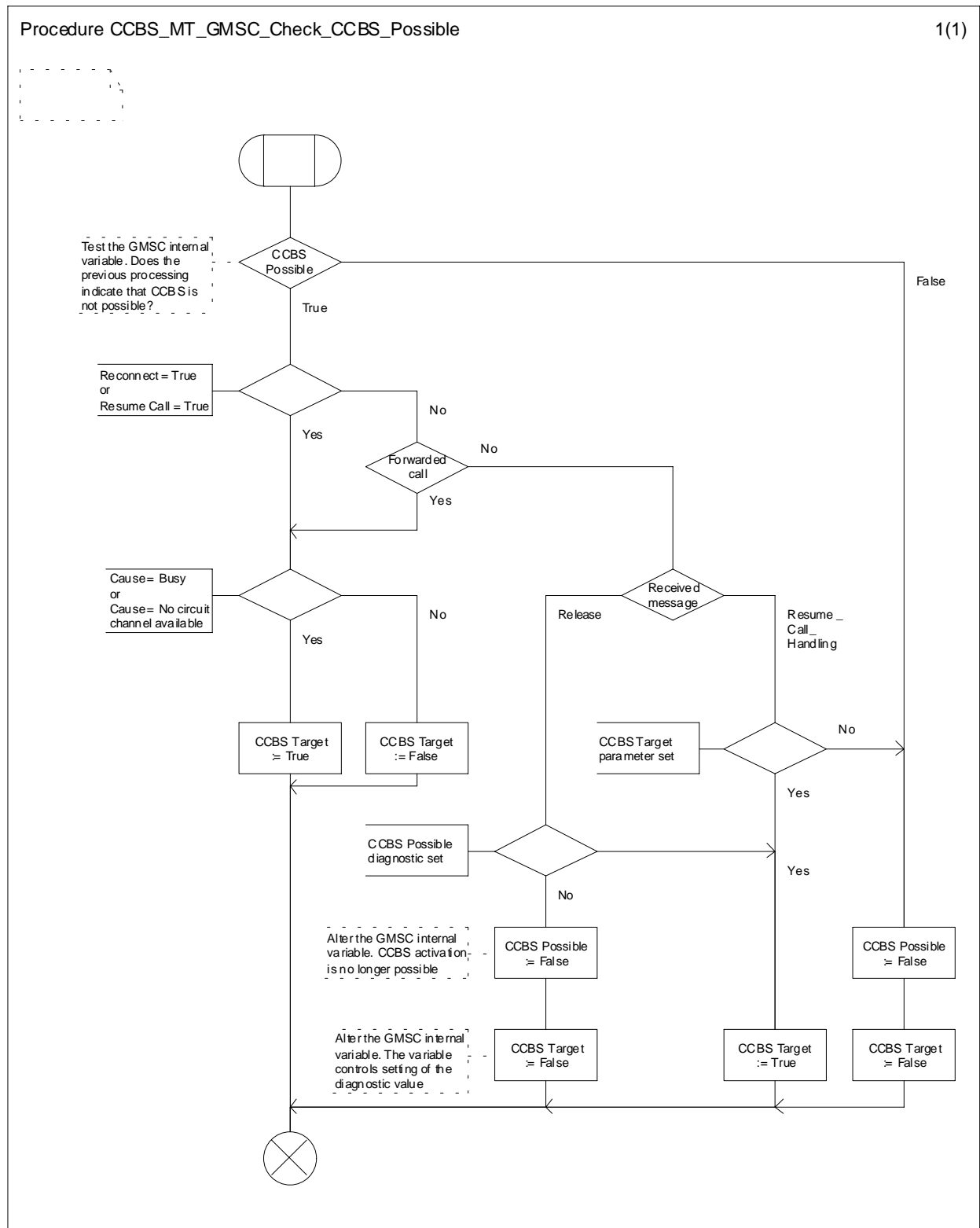
Figure 11.2.1.5: Procedure CCBS_MT_GMSC_Check_CCBS_Possible
