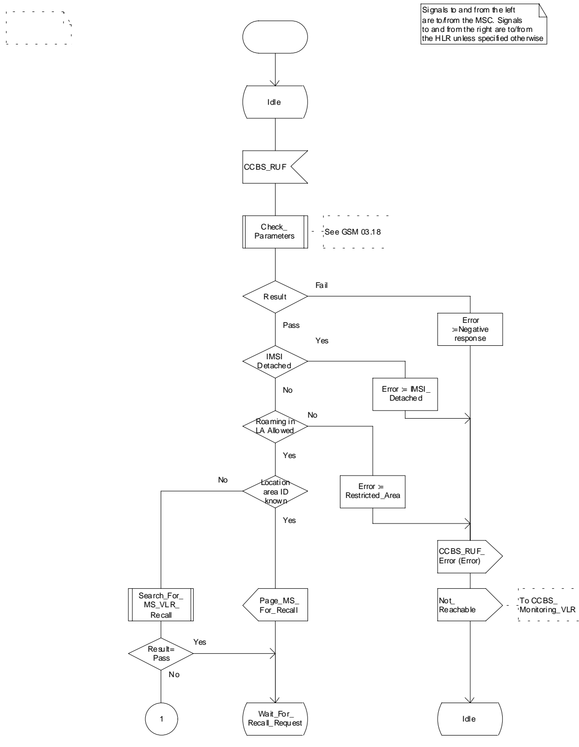
Figure 11.1.1.2: Process VLR_CCBS_Recall_Manager (sheet 1 of 4)
