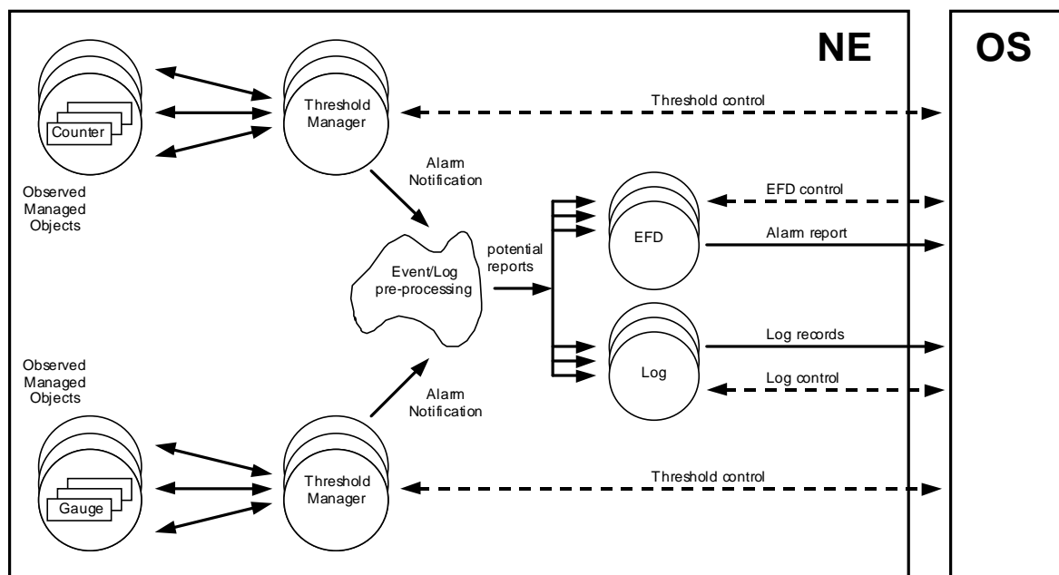
Figure 2: Inter-relationship of counters and gauges with thresholds
