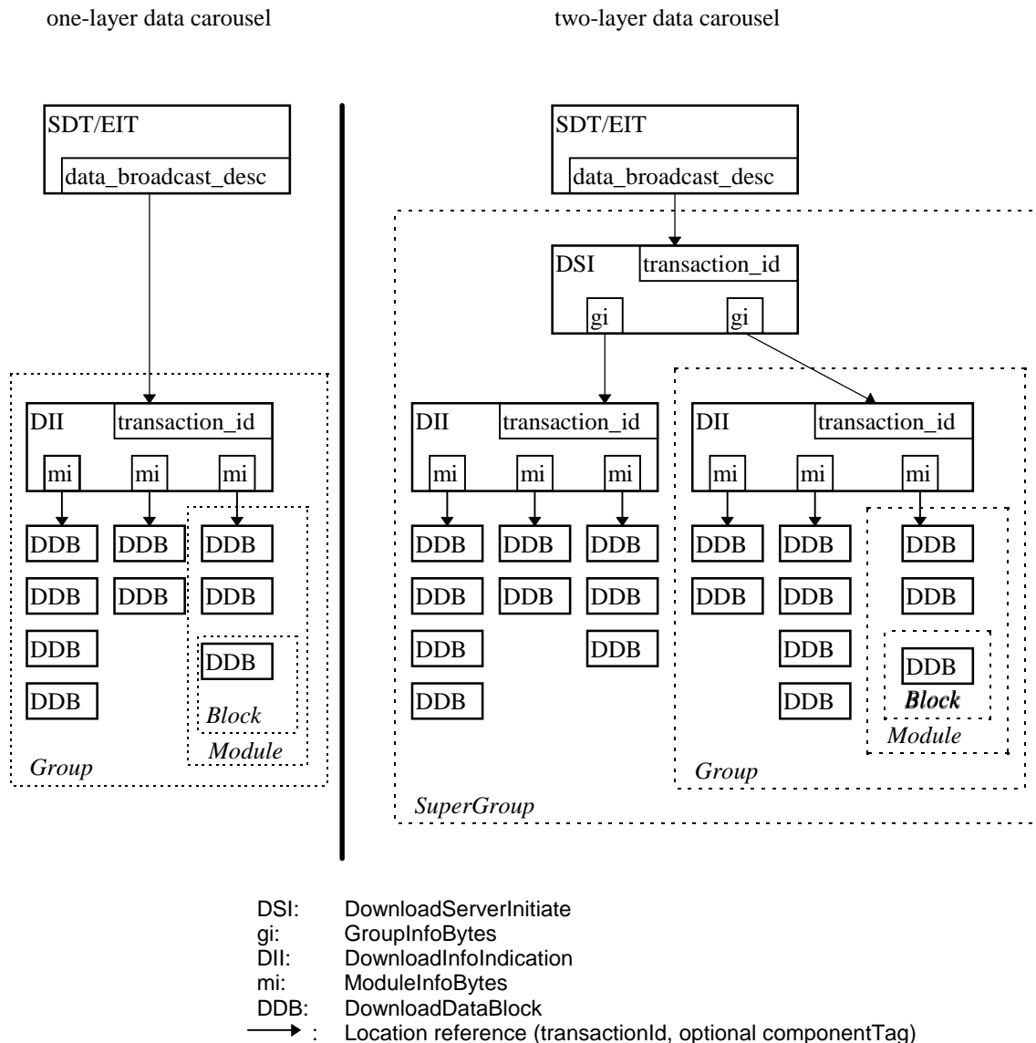
Figure 2: Structure of the DVB data carousel
