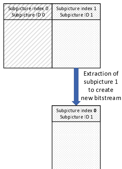
Figure M.1: VVC subpictures extraction
